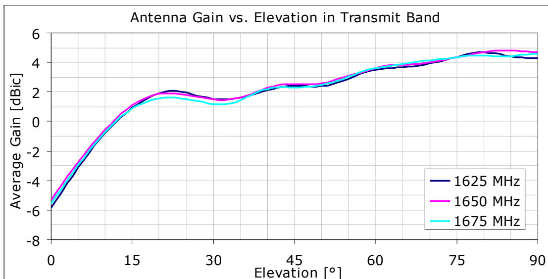
Figure 6. Gain vs Elevation for AT1595-90, SN3002 antenna for Inmarsat transmit band. 0° and 90° elevations correspond to antenna horizon and zenith, respectively.
