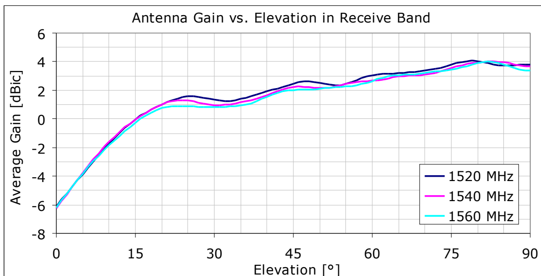
Figure 5. Gain vs Elevation for AT1595-90, SN3002 antenna for Inmarsat receive band. 0° and 90° elevations correspond to antenna horizon and zenith, respectively.
