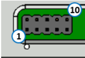
Figure 22. Audio pin header interface pin organization
