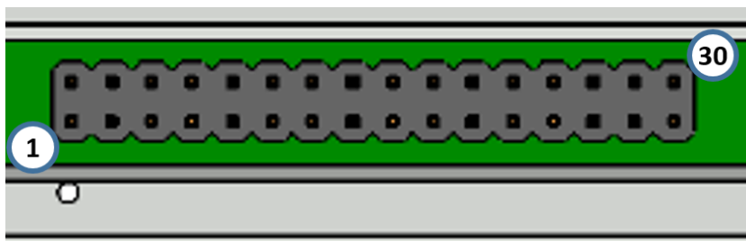
Figure 20. VAM control interface pin organization
