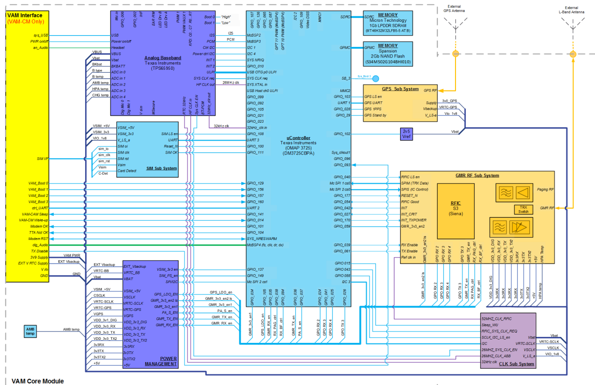
Figure 3. Block diagram of IsatPhone 2v1 VAM-CM
