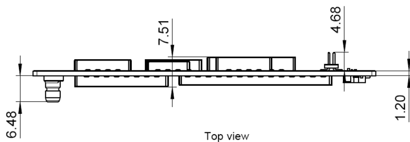
Figure 12. Side view dimensions
