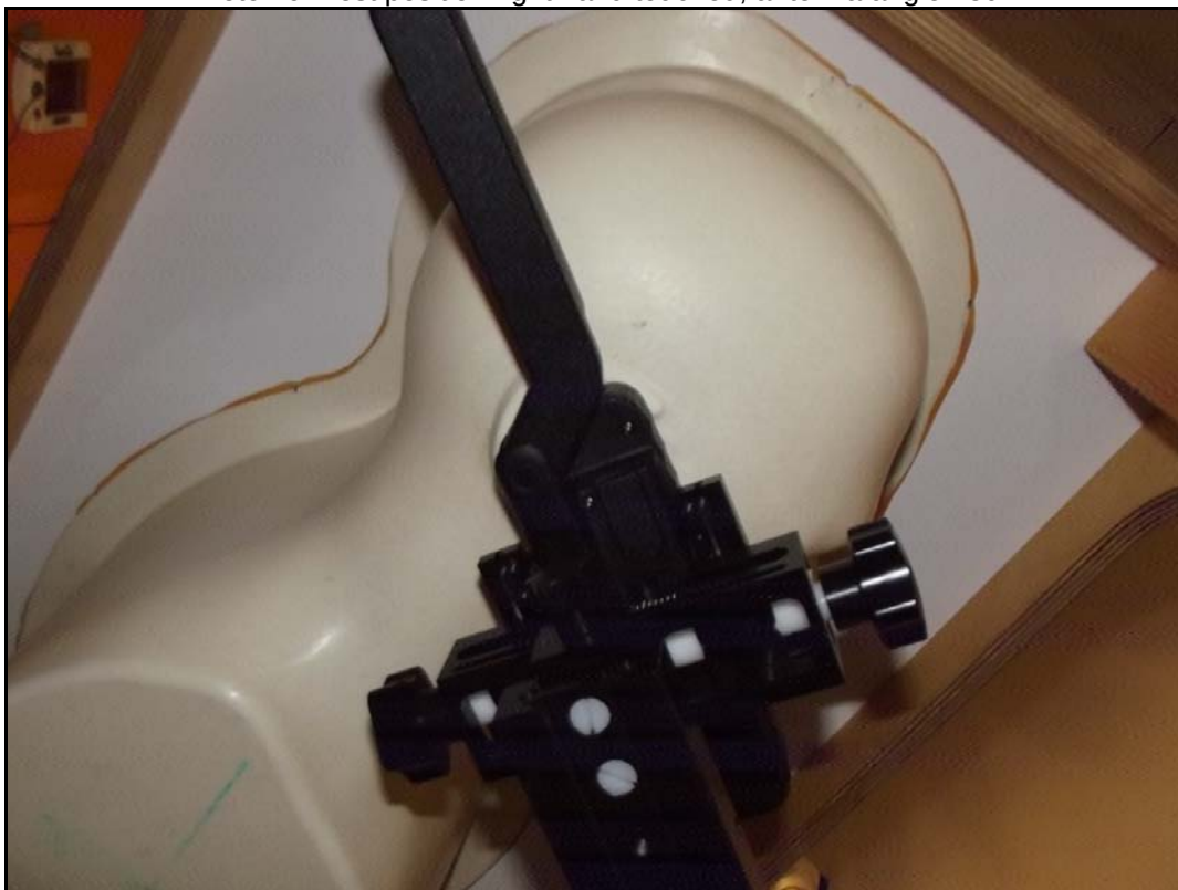
Photo 20: Test position right hand touched, antenna angle 225°
