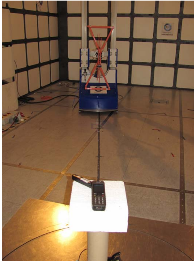
Radiated Emissions 30MHz-1GHz
