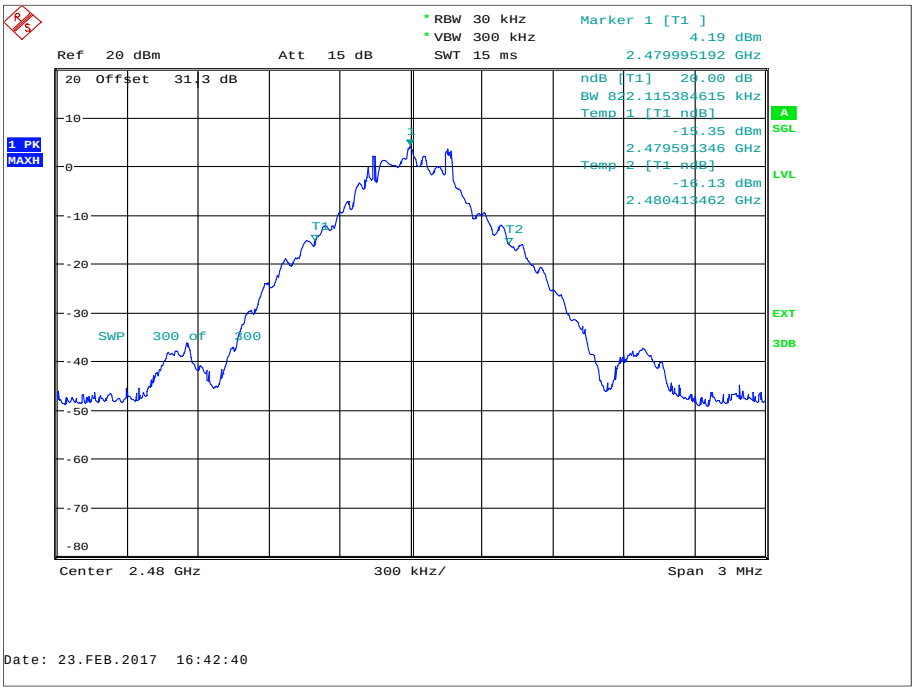
Figure 19 – 2480 MHz - GFSK
