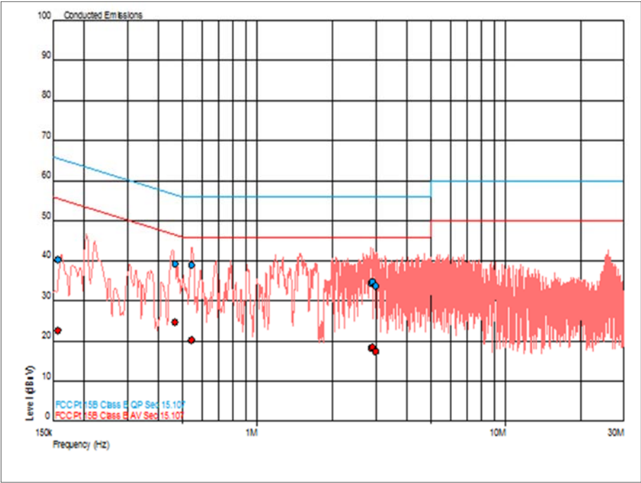
Figure 1 – Live Line
