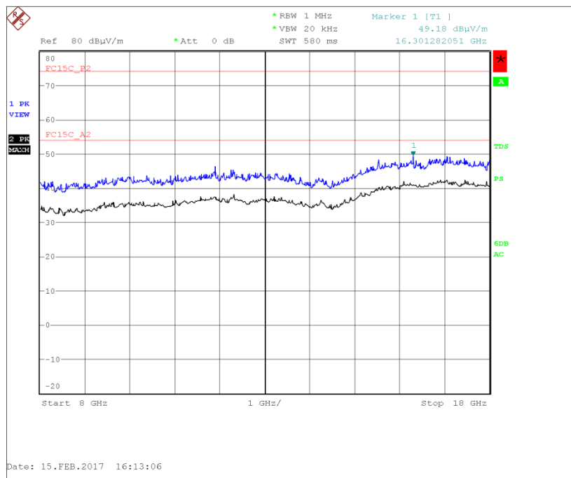
Figure 30 - 8 GHz to 18 GHz - Horizontal and Vertical
