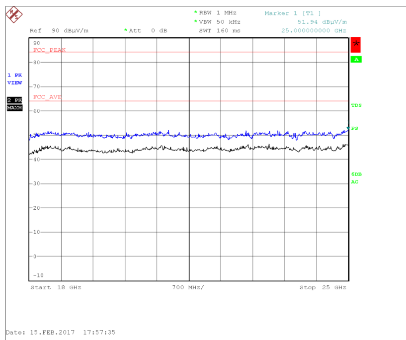
Figure 26 - 18 GHz to 25 GHz - Horizontal and Vertical
