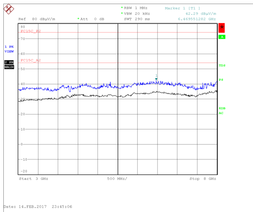
Figure 34 - 3 GHz to 8 GHz - Horizontal and Vertical
