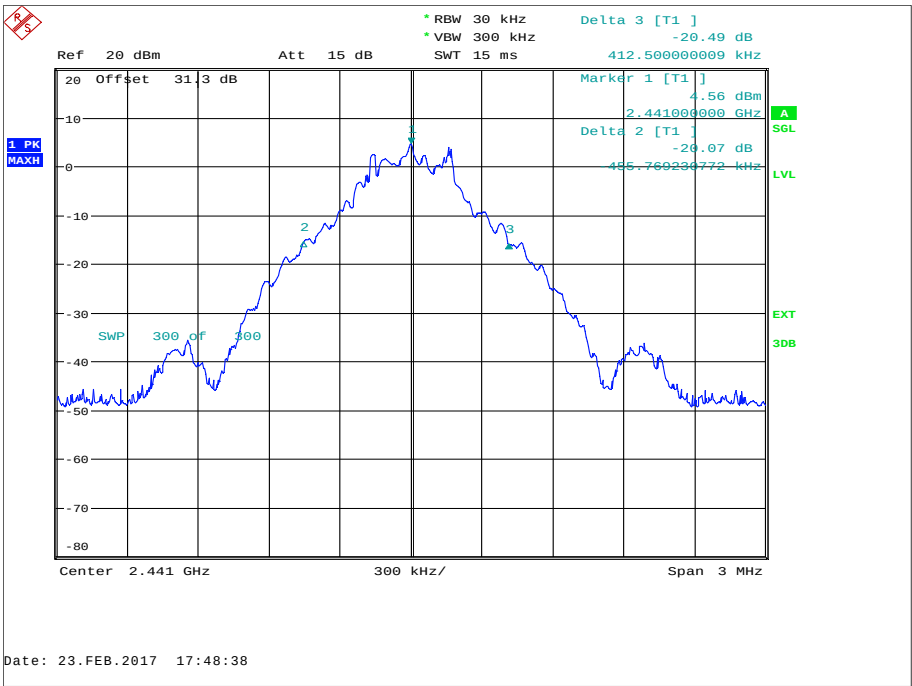
Figure 16 - 2441 MHz - GFSK
