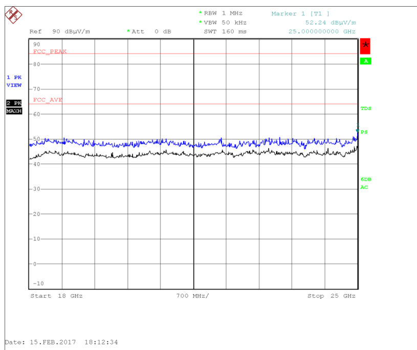
Figure 31 - 18 GHz to 25 GHz - Horizontal and Vertical
