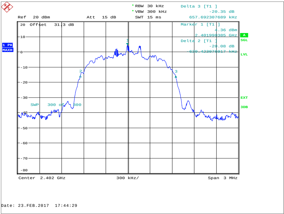
Figure 15 – 2402 MHz - 8-DPSK
