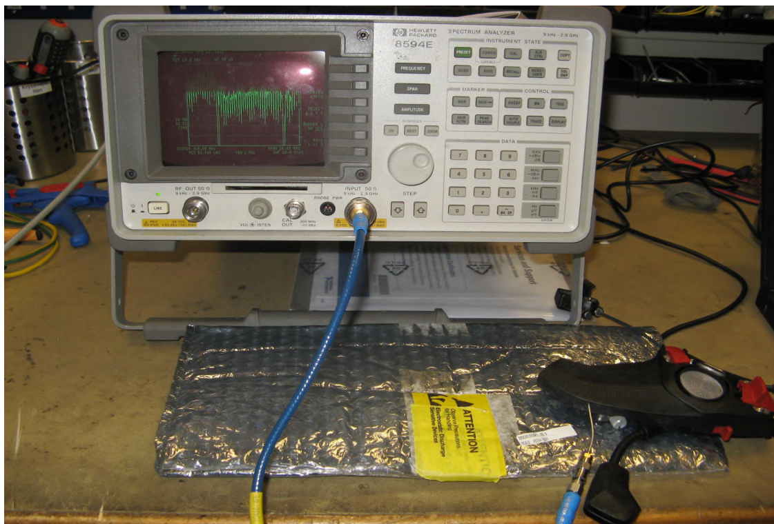
Photo 4.2.1 Test setup regarding measurement of hopping channels.
