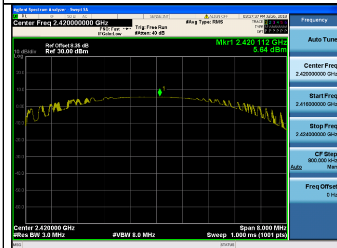
GFSK Output power - High CH 2420
