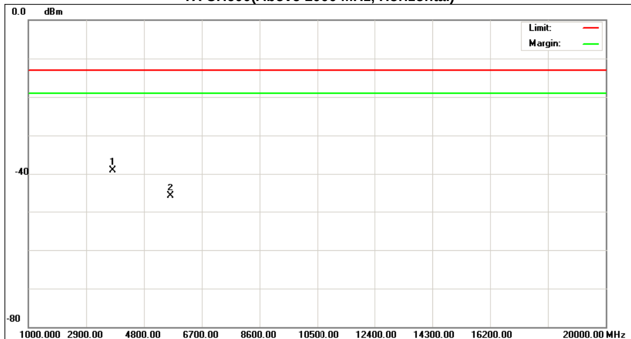
TX CH600(Above 1000 MHz, Horizontal)
