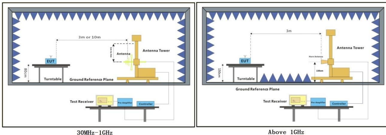
30MHz-1GHz
