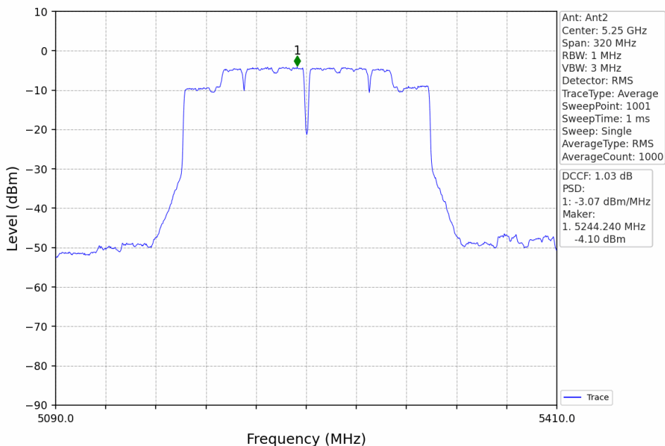
802.11ac(VHT160)_MCH_5250MHz_Ant2_NTNV
