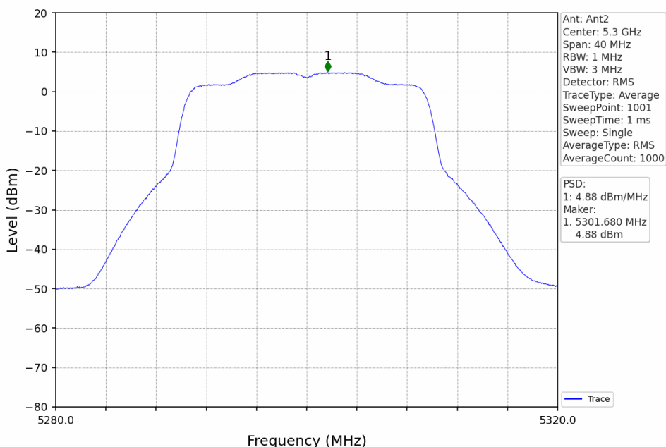
802.11ax(HEW20)_MCH_5300MHz_RU242_Left_MIMO_NTNV
