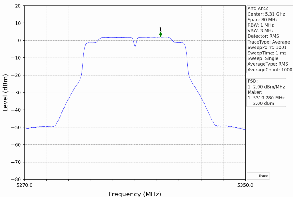
802.11ac(VHT40)_HCH_5310MHz_MIMO_NTNV
