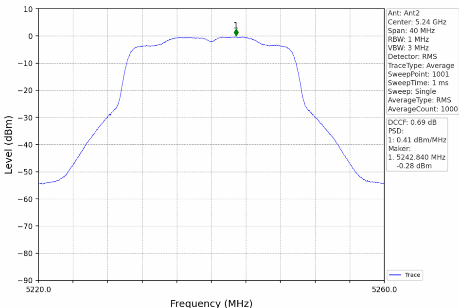
802.11ax(HEW20)_HCH_5240MHz_RU242_Left_MIMO_NTNV
