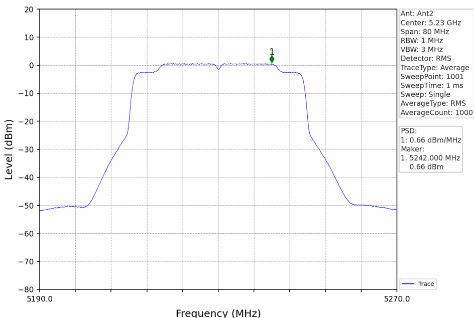
802.11ax(HEW40)_HCH_5230MHz_RU484_Left_MIMO_NTNV
