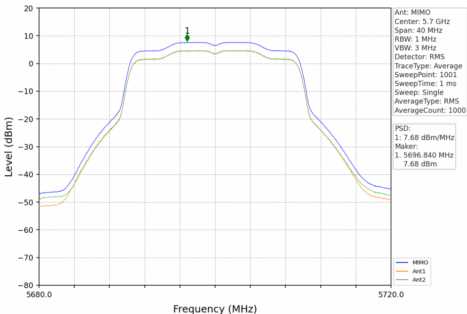
802.11ax(HEW20)_HCH_5700MHz_RU242_Left_MIMO_NTNV
