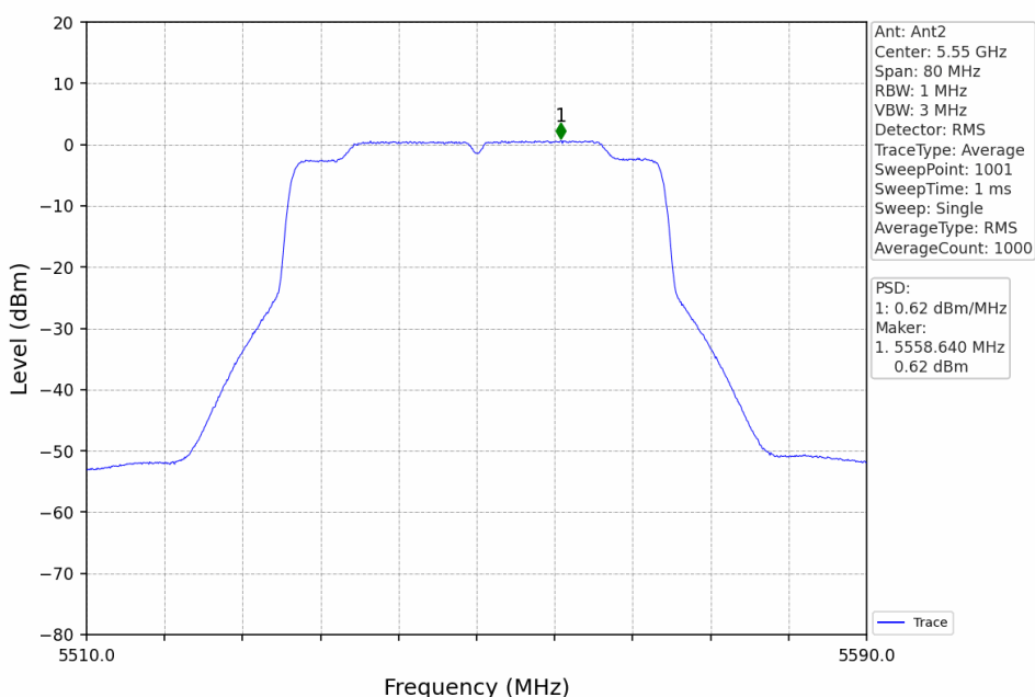
802.11ax(HEW40)_MCH_5550MHz_RU484_Left_MIMO_NTNV
