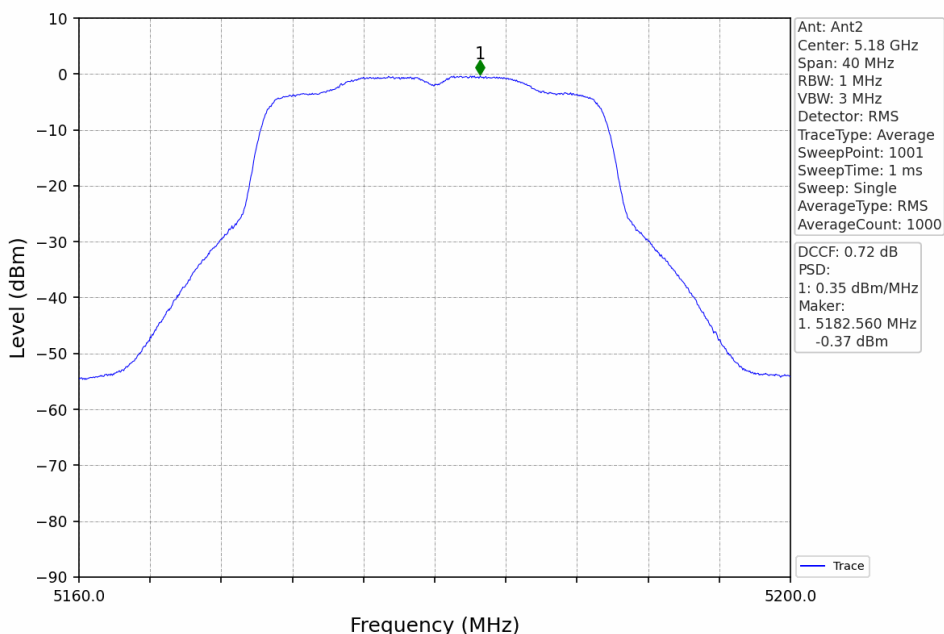
802.11ax(HEW20)_LCH_5180MHz_RU242_Left_MIMO_NTNV
