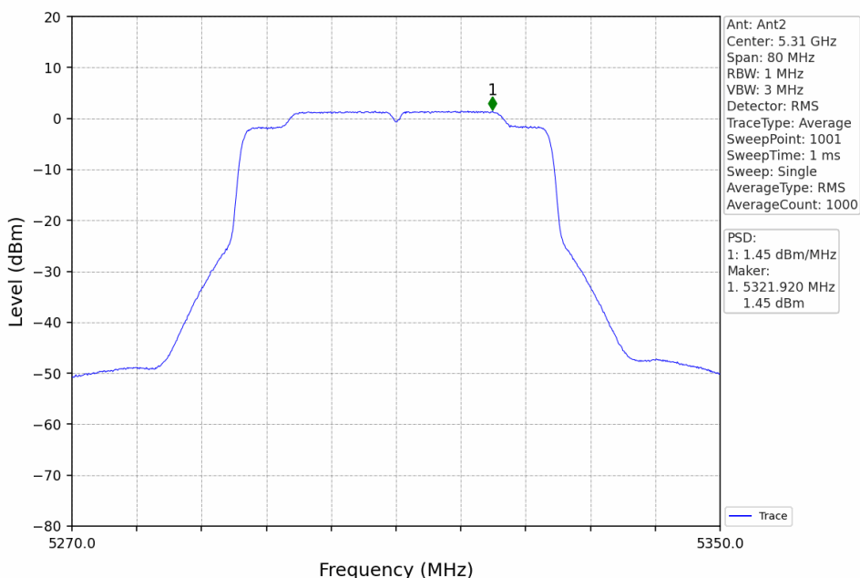
802.11ax(HEW40)_HCH_5310MHz_RU484_Left_MIMO_NTNV
