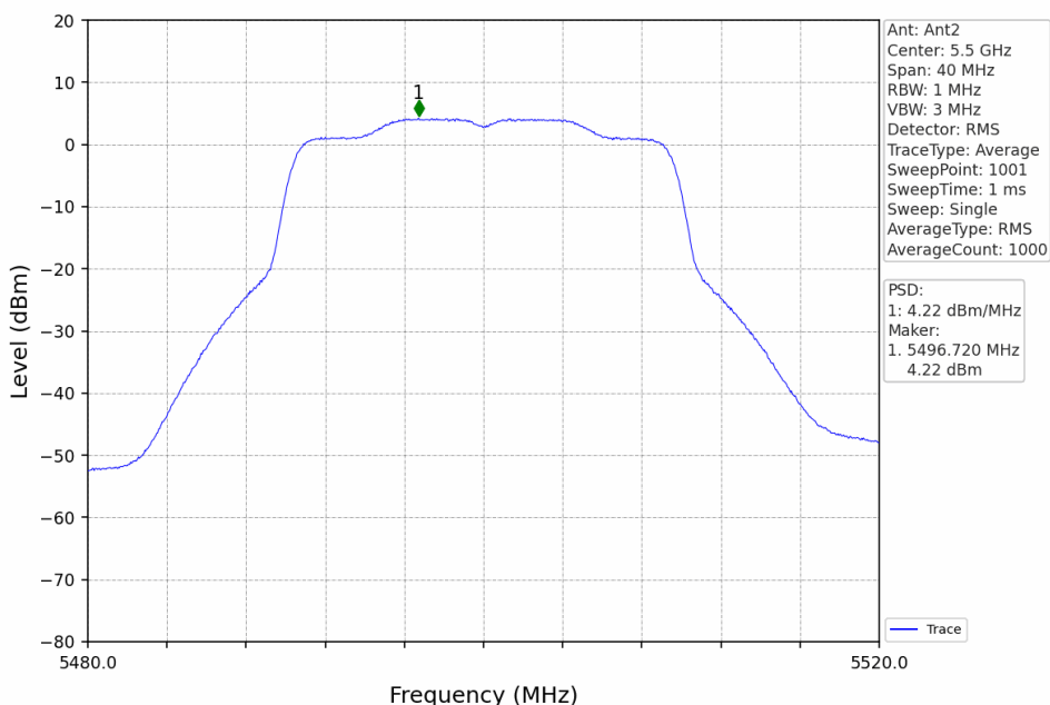
802.11ax(HEW20)_LCH_5500MHz_RU242_Left_MIMO_NTNV
