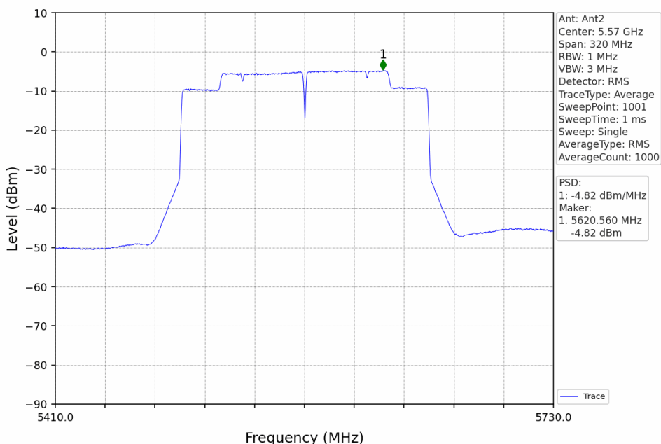
802.11ax(HEW160)_MCH_5570MHz_2xRU996_Left_MIMO_NTNV
