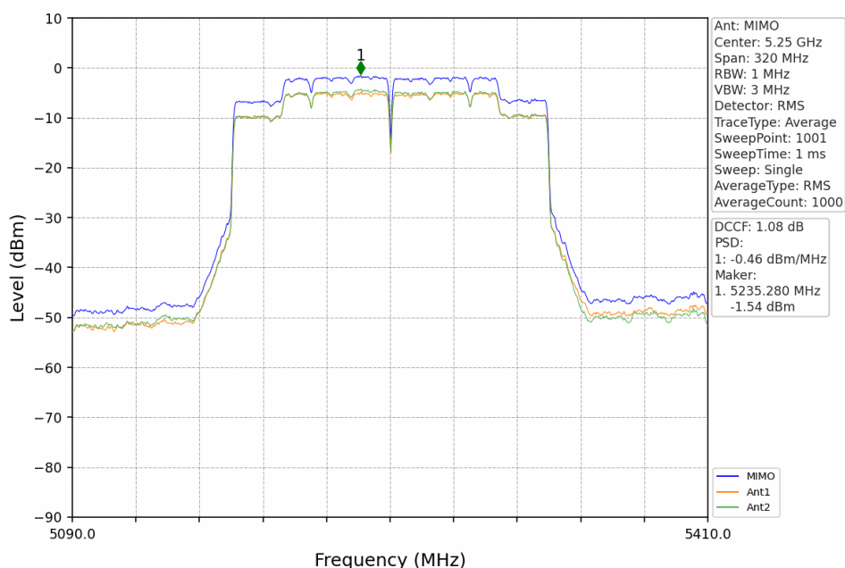
802.11ax(HEW160)_MCH_5250MHz_2xRU996_Left_MIMO_NTNV
