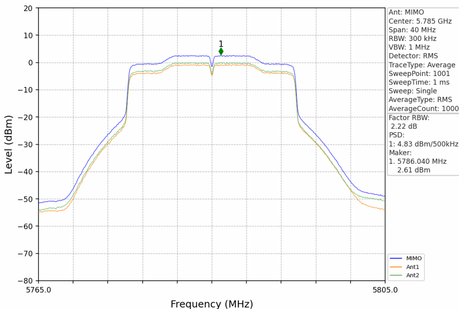
802.11ax(HEW20)_MCH_5785MHz_RU242_Left_MIMO_NTNV
