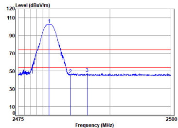
BT_DH5_TX_CH_78_Vertical
