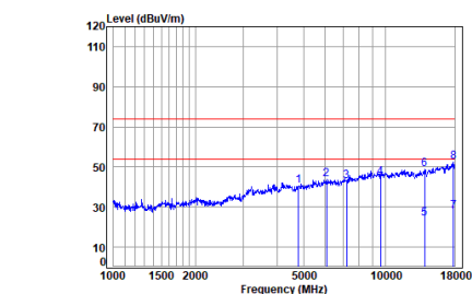
BT_DH5_TX_CH_00_Horizontal
