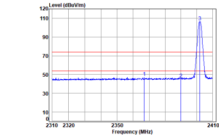
BT_DH5_TX_CH_00_Horizontal
