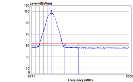
BT_DH5_TX_CH_78_Horizontal
