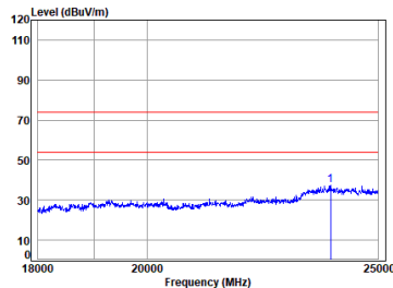
BT_TX_CH_M_Horizontal
