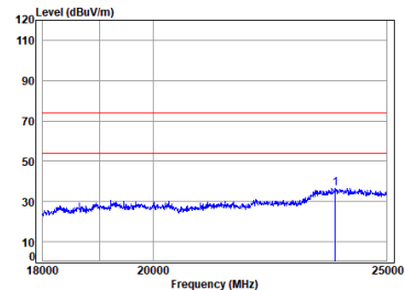
BT_TX_CH_M_Vertical
