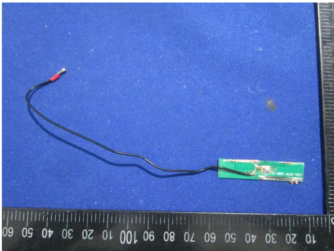
WiFi Antenna-1
