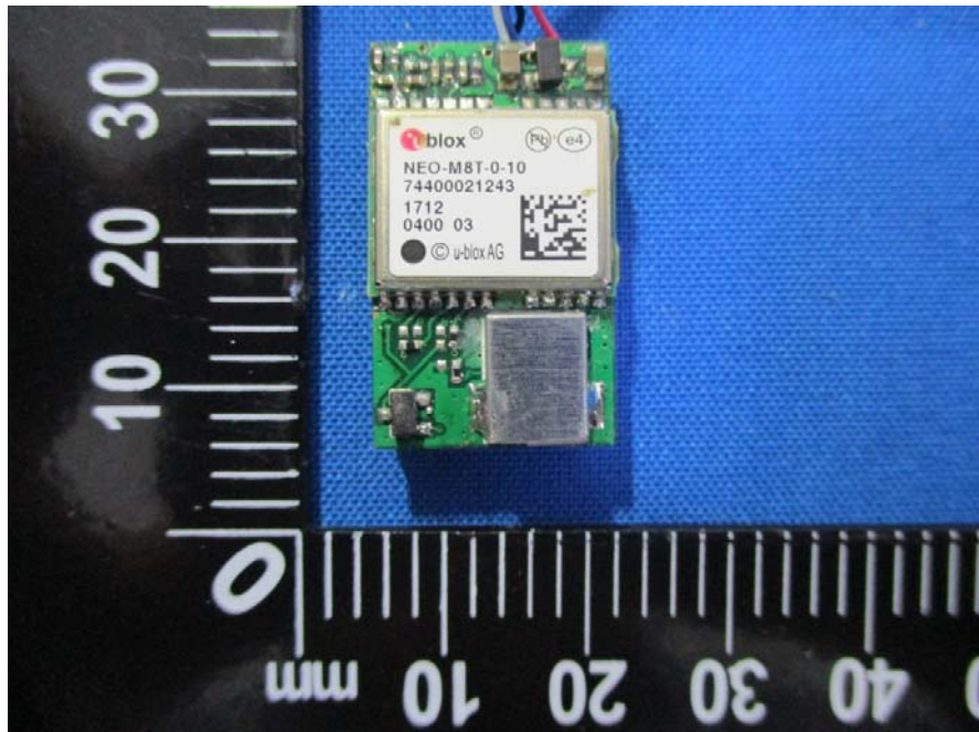
EUT –GPS Module With Antenna Top View
