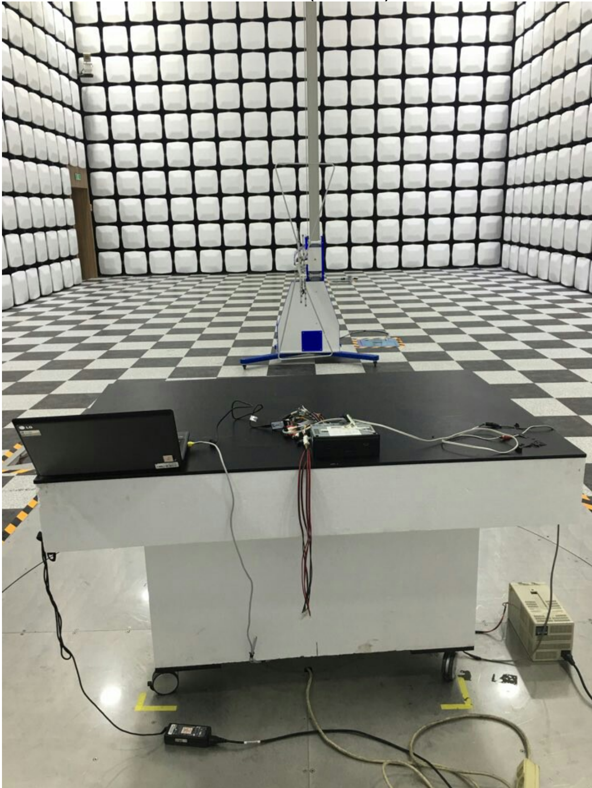
Radiated Test(1G below)
