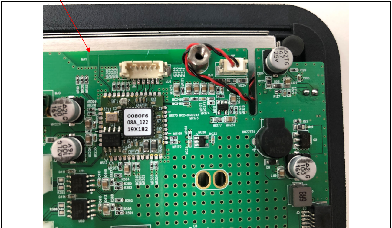
PCB Antenna
