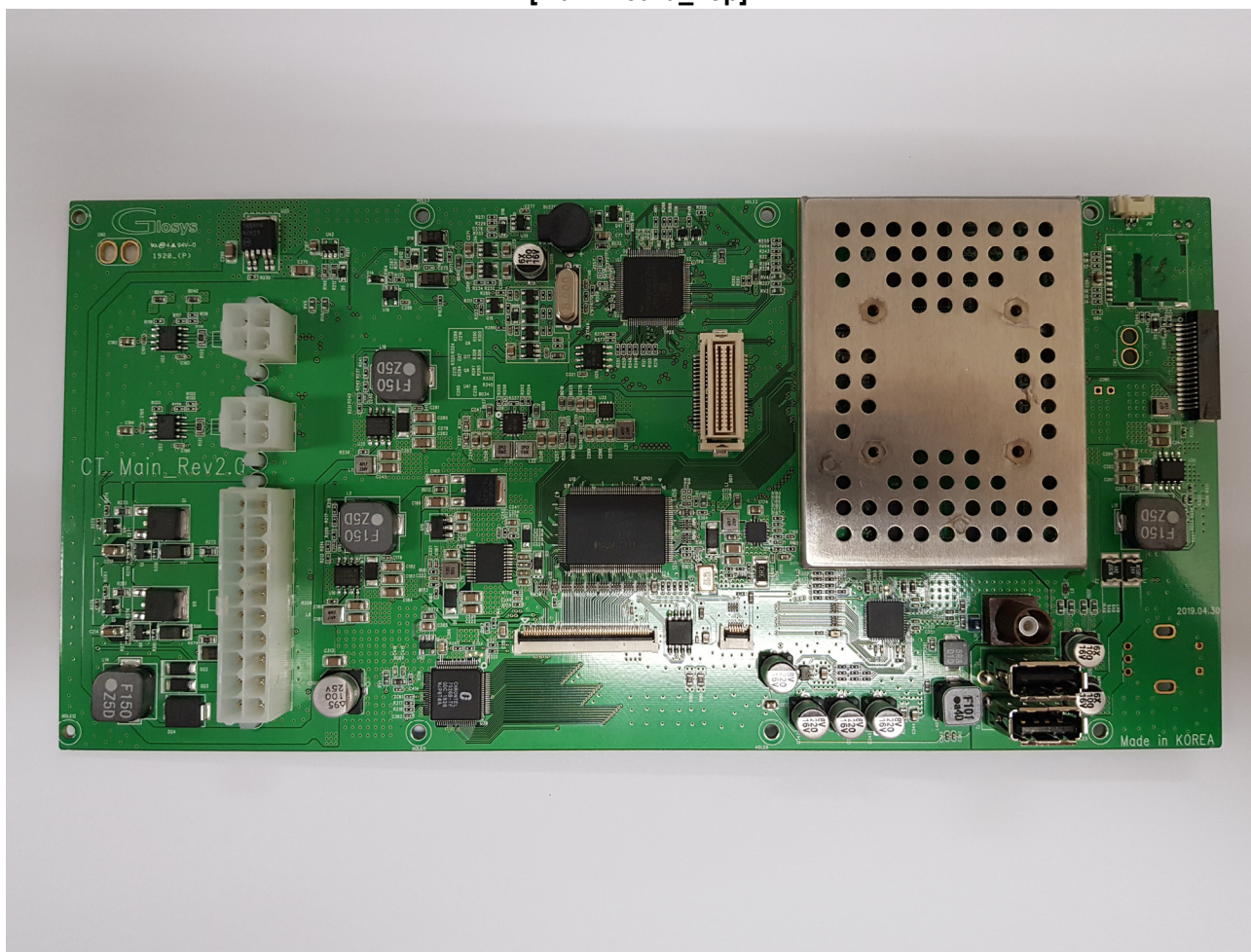
[Main Board_Top]
