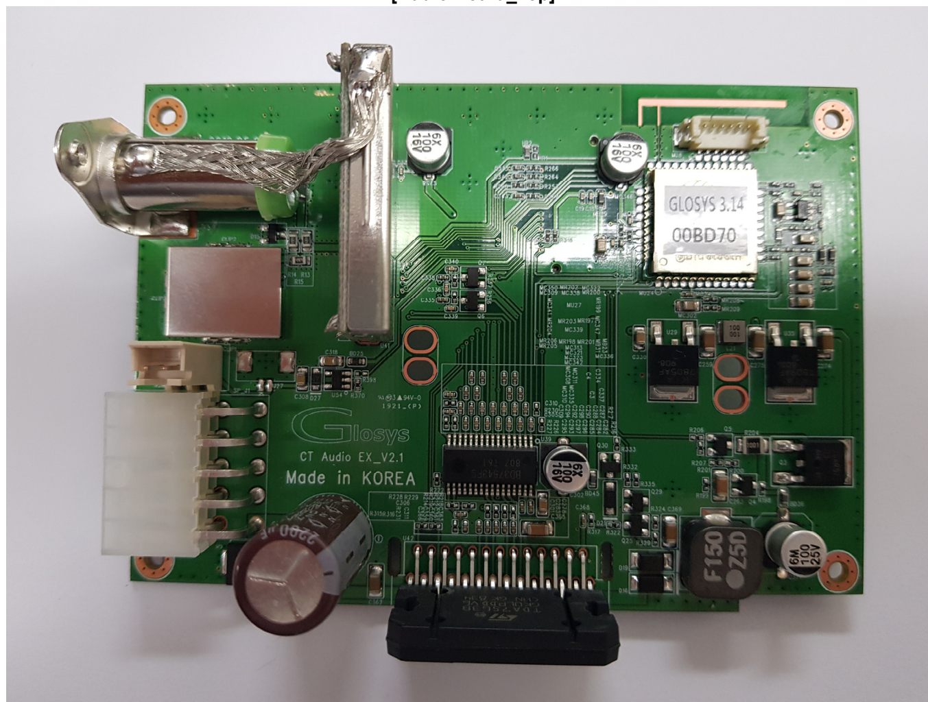
[Audio Board_Top]
