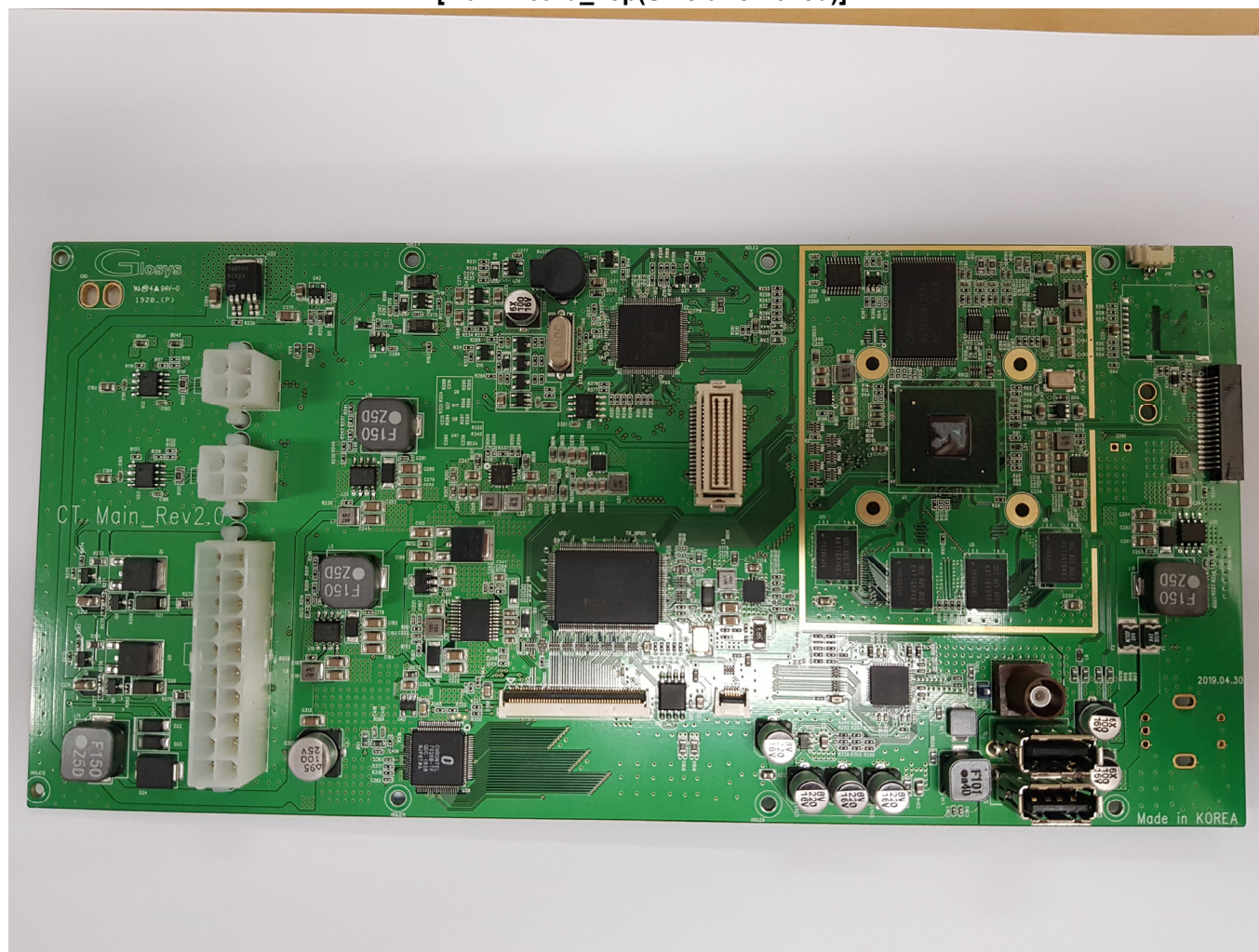
[Main Board_Top(Shield removed)]
