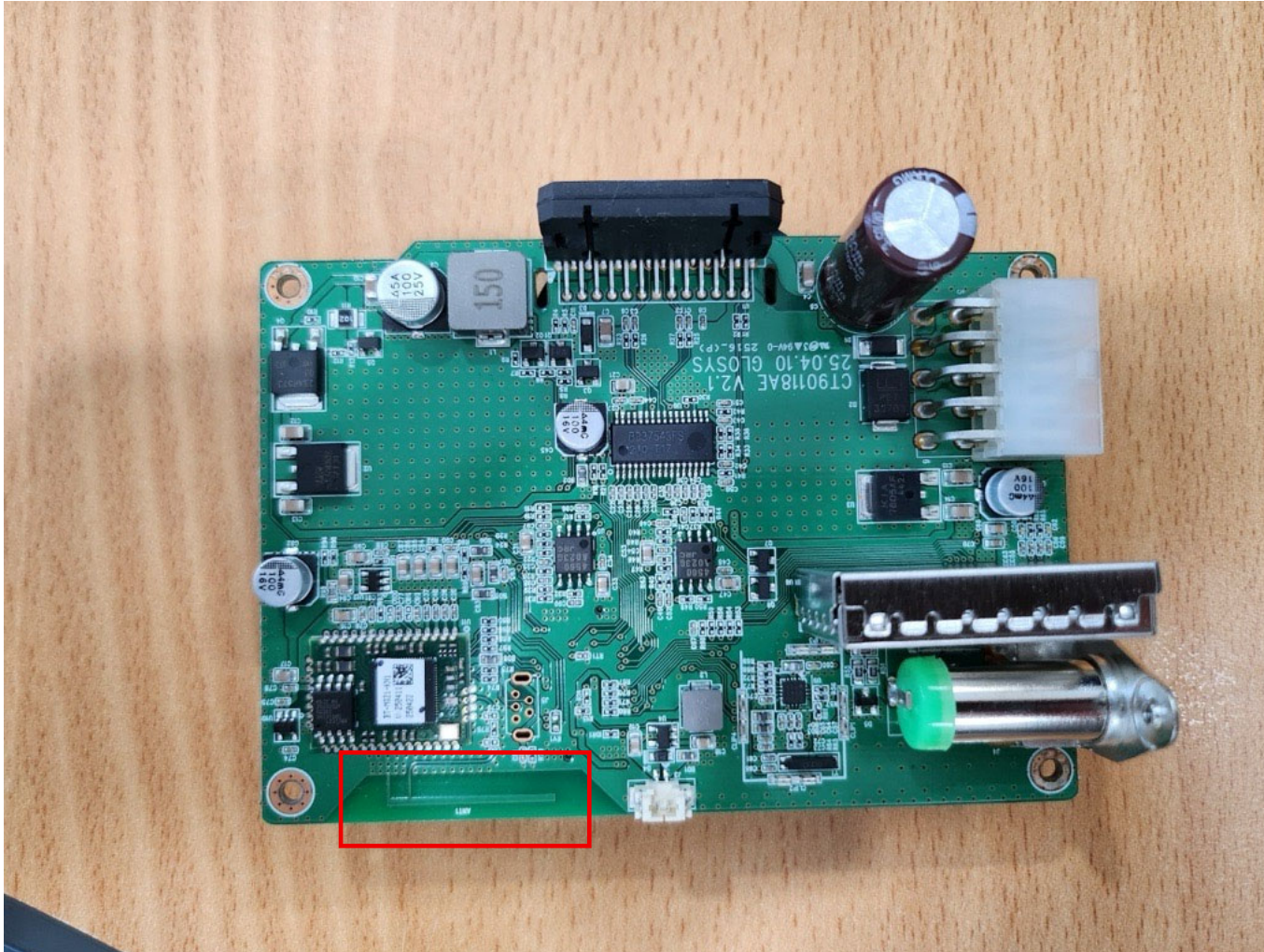
[Main board_Top]
