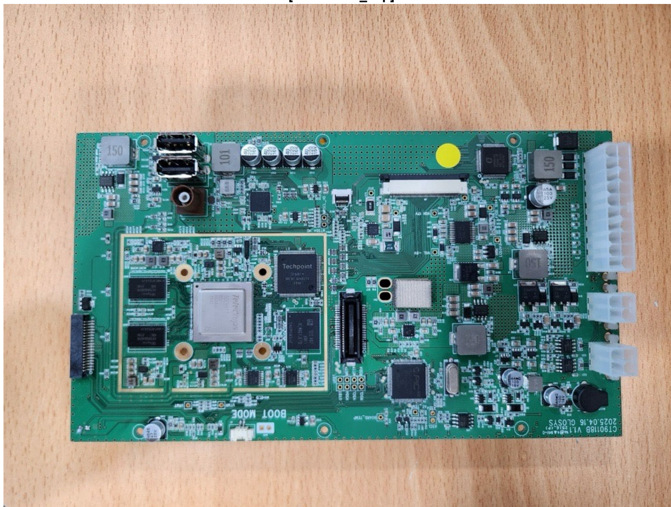
[Sub Board_Top]
