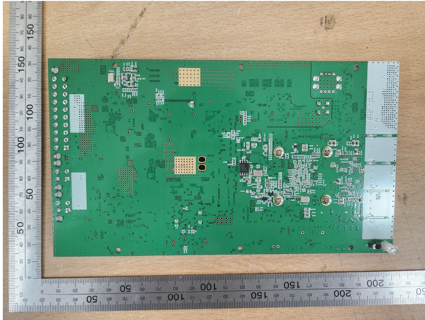
[Sub Board_Bottom]
