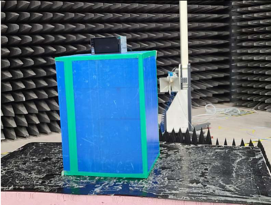
18 GHz – 25 GHz
