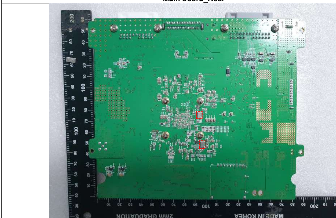
Main board_Rear
