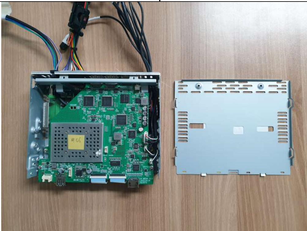
Main board_front
