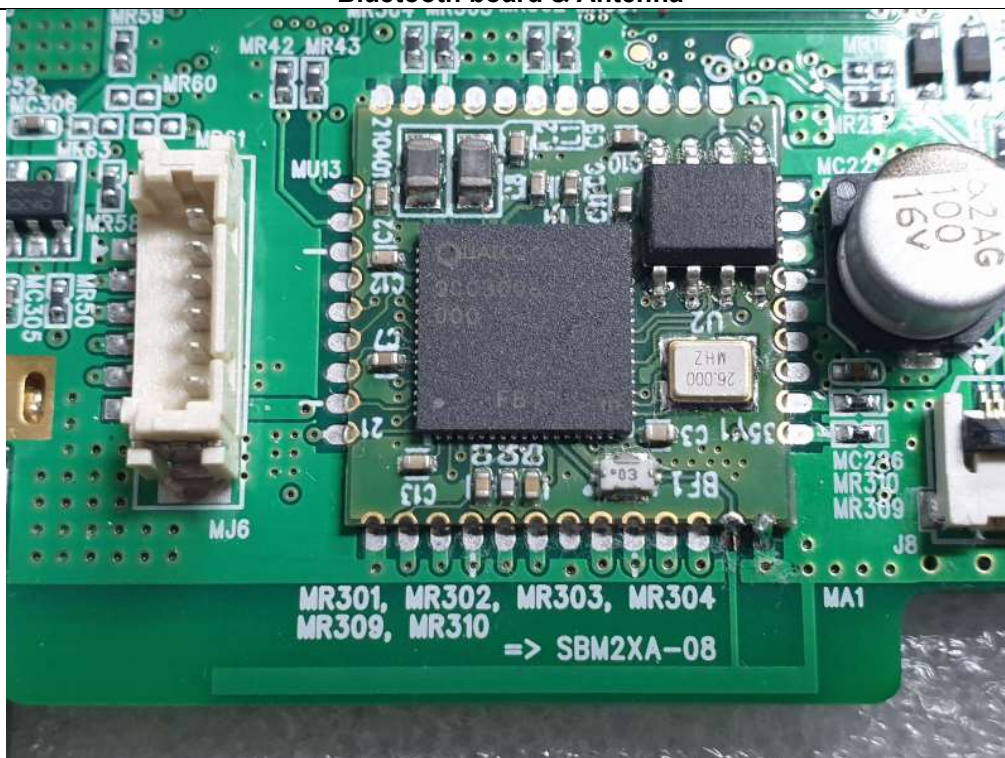
Bluetooth board & Antenna
