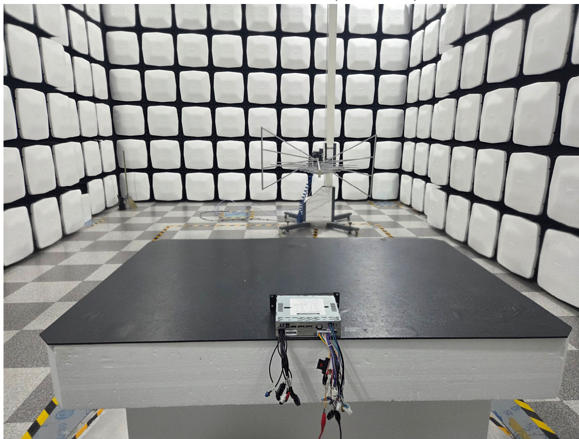
Radiated RF measurement (Below 1 GHz)
