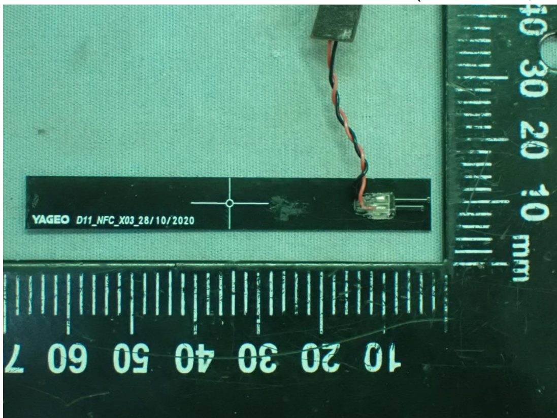
Figure 16 Internal View (NFC Antenna, Back View)
