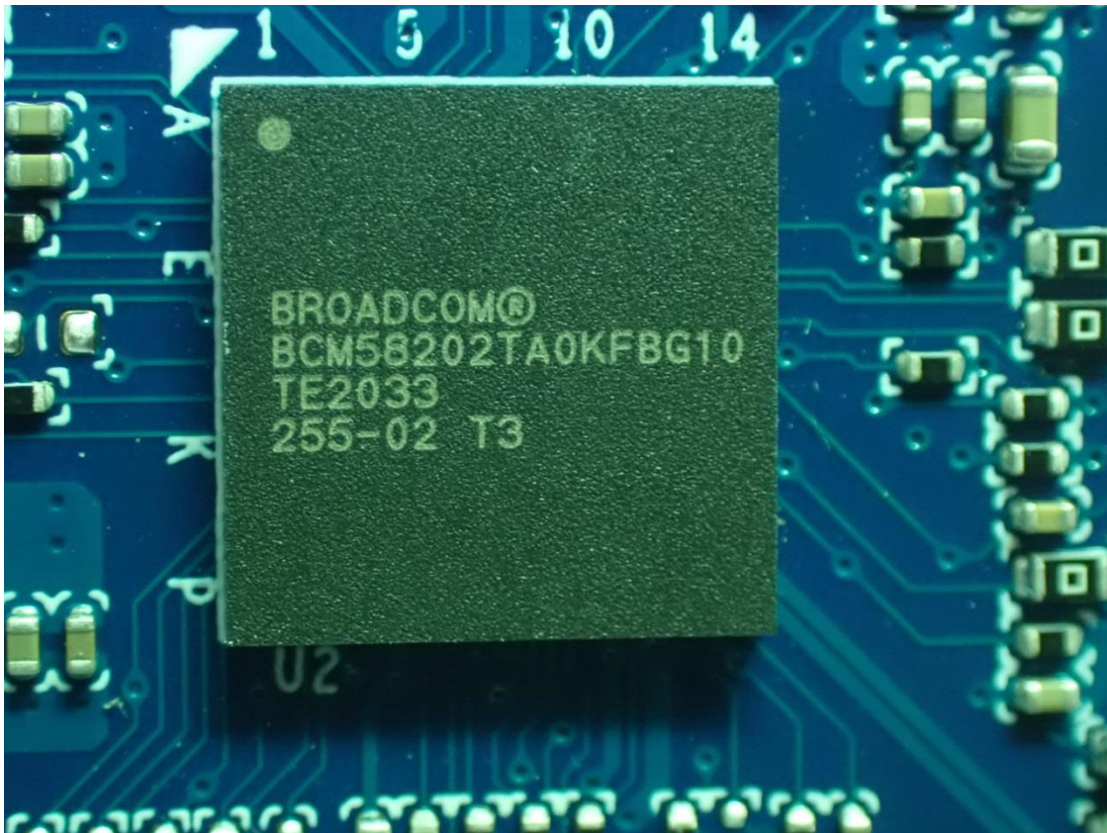
Figure 11 Internal View (NFC Chip View)
