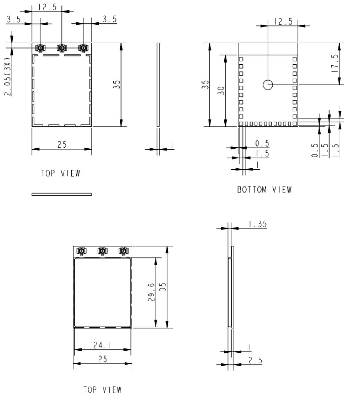
Figure 3 Mechanical Drawing
