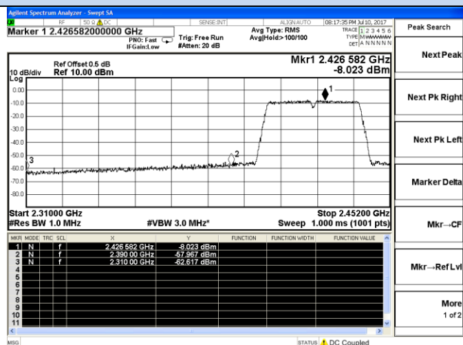
Channel 3 / 2422 MHz – Peak
