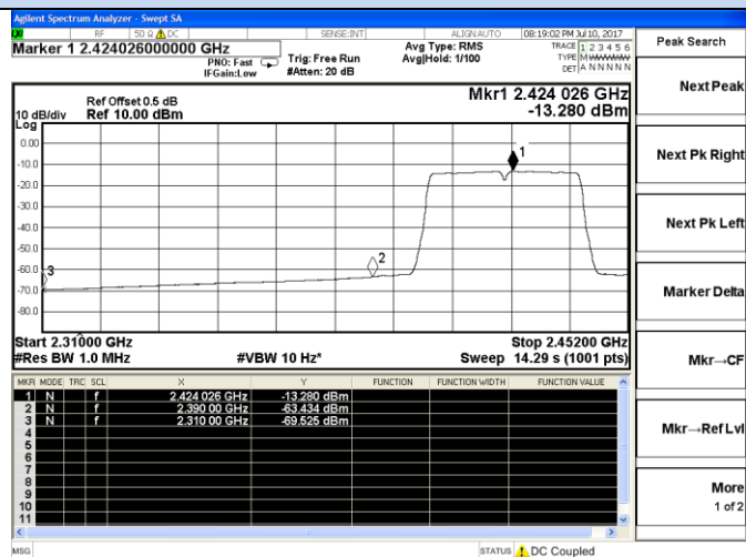
Channel 3 / 2422 MHz – Average
