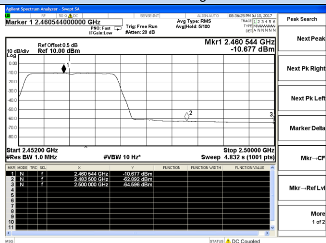
Channel 11 / 2462 MHz – Average
