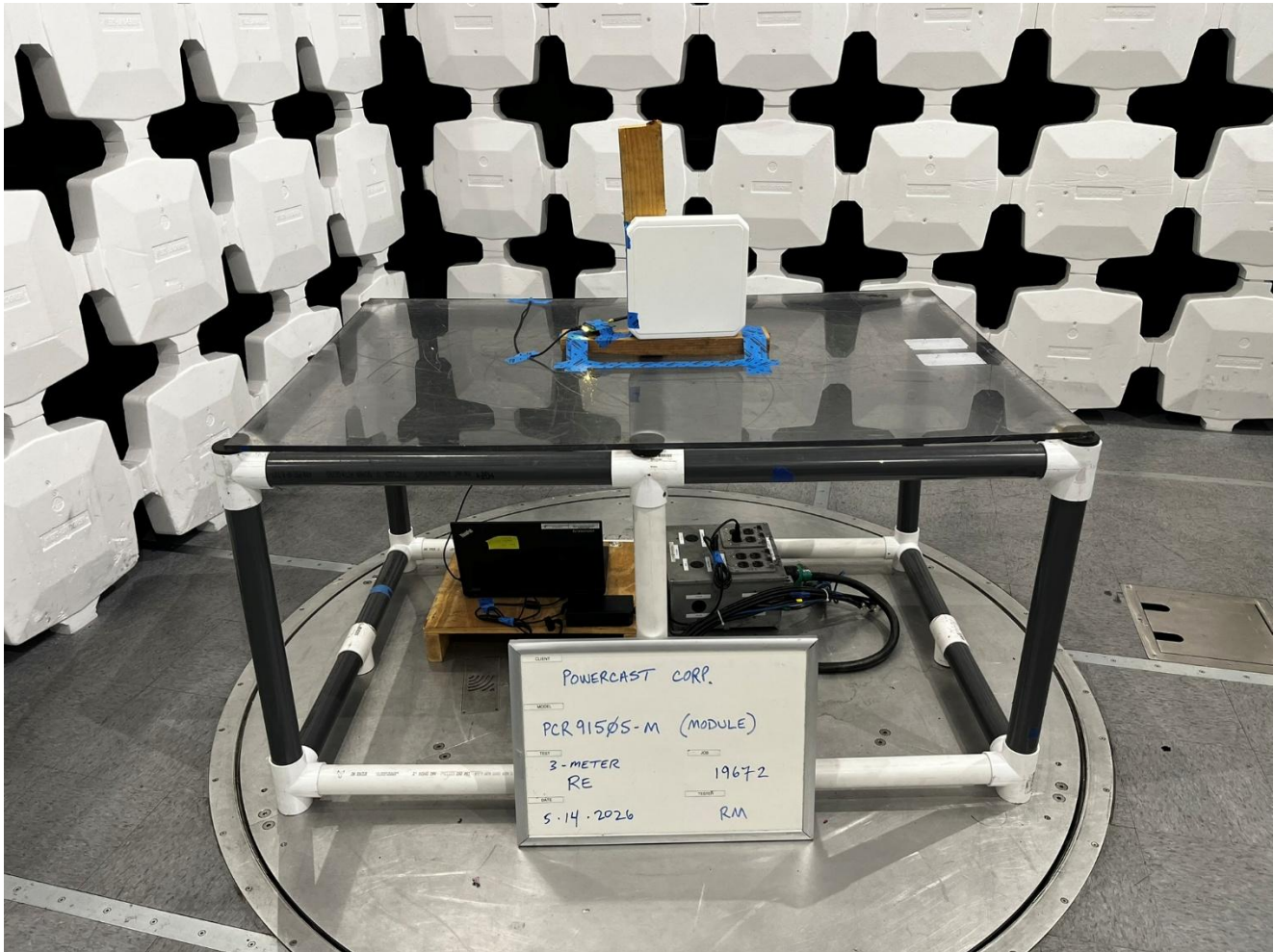
Antenna #2: PAR90209H, Radiated Emissions, 30MHz to 1GHz, View 2
