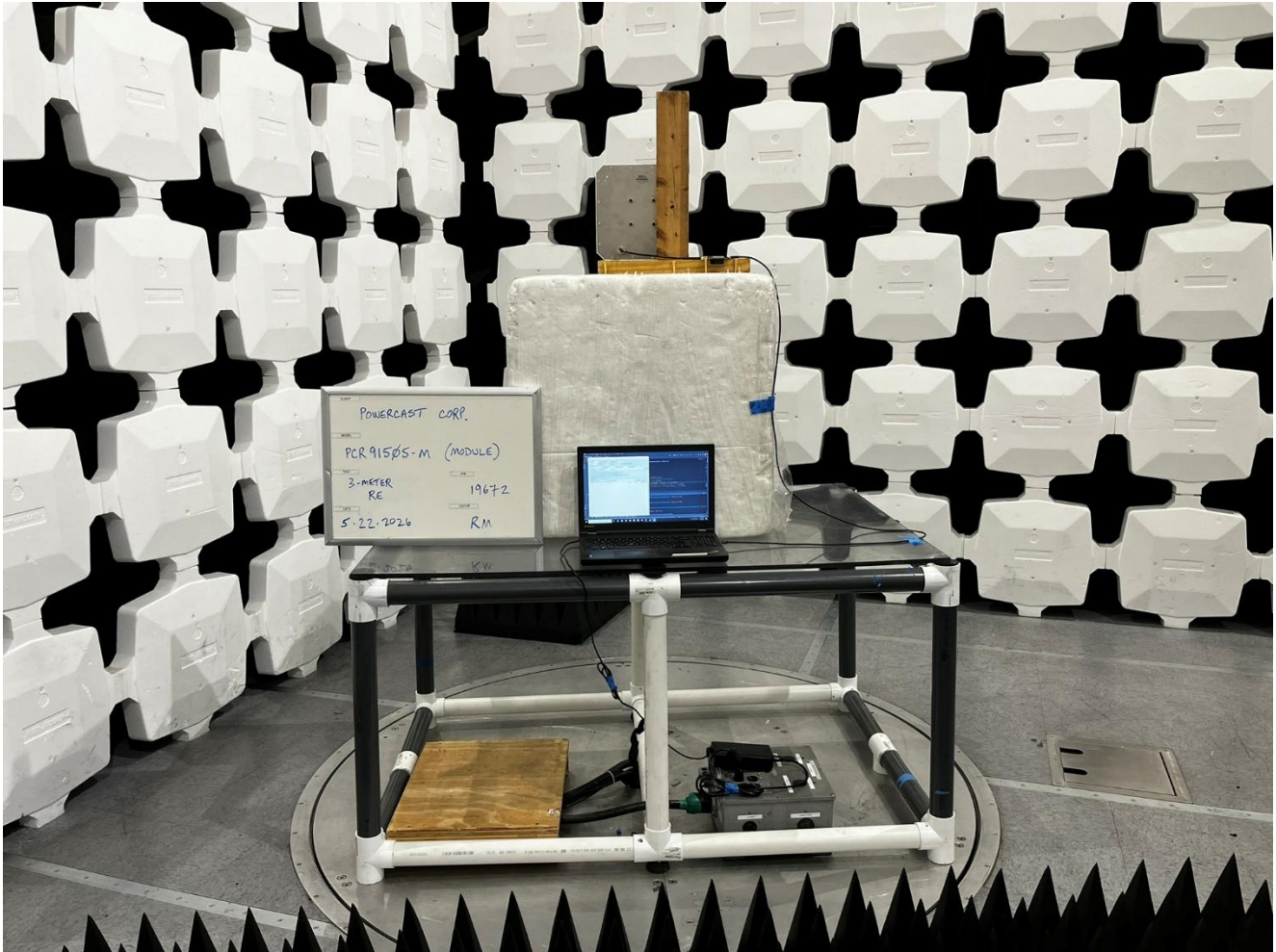
Antenna #2: PAR90209H, Radiated Emissions, 1GHz to 9.3GHz, View 3
