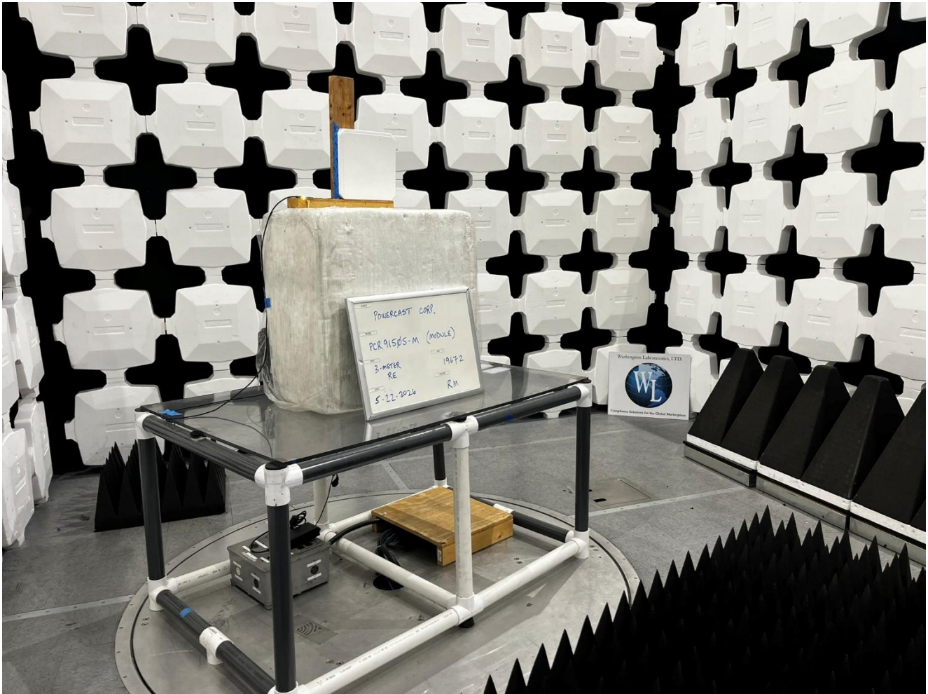
Antenna #2: PAR90209H, Radiated Emissions, 1GHz to 9.3GHz, View 2
