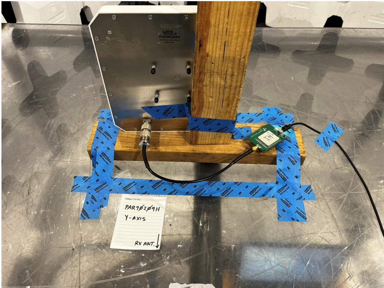
Antenna #2: PAR90209H, Radiated Emissions, 30MHz to 1GHz, View 4
