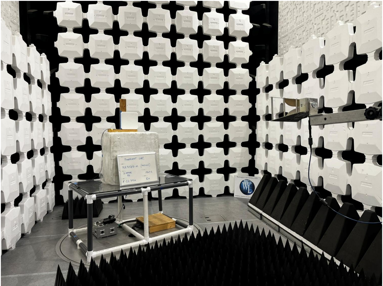
Antenna #2: PAR90209H, Radiated Emissions, 1GHz to 9.3GHz, View 1
