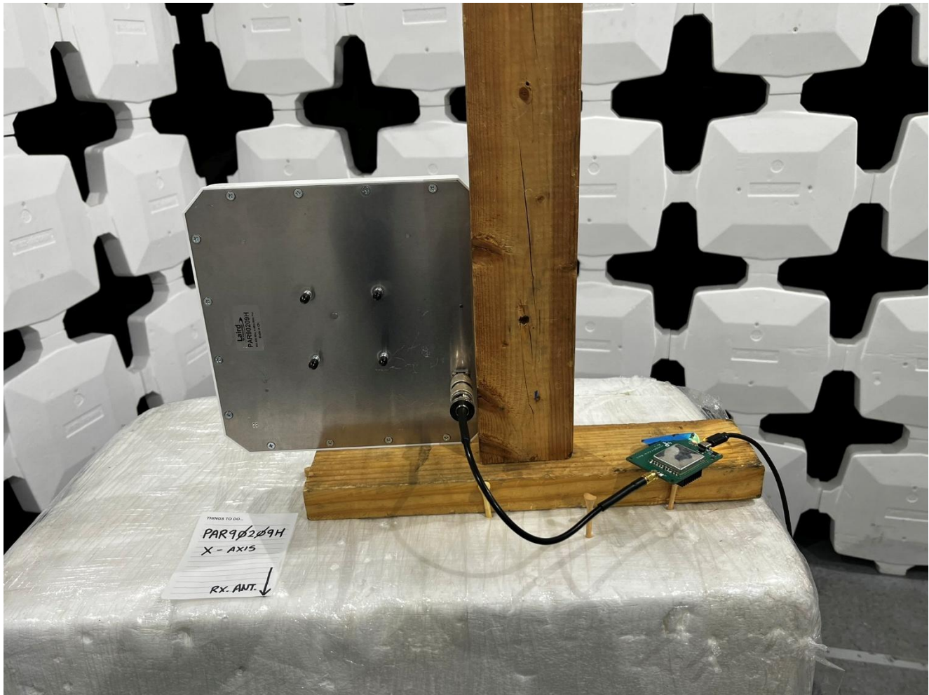
Antenna #2: PAR90209H, Radiated Emissions, 1GHz to 9.3GHz, View 4
