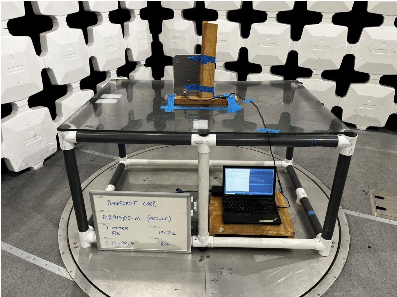
Antenna #2: PAR90209H, Radiated Emissions, 30MHz to 1GHz, View 3
