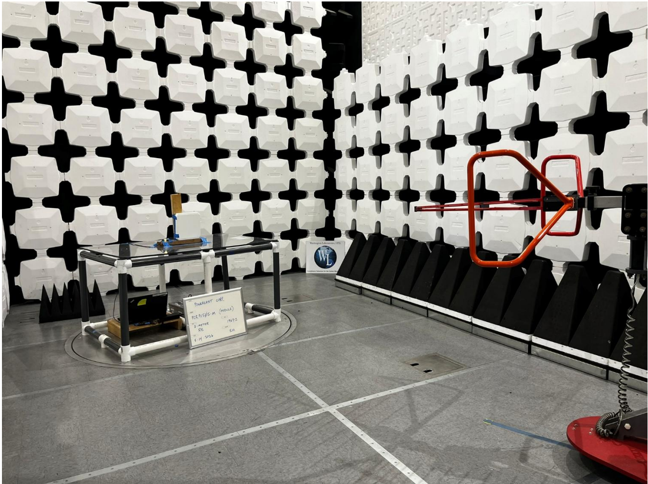
Antenna #2: PAR90209H, Radiated Emissions, 30MHz to 1GHz, View 1
