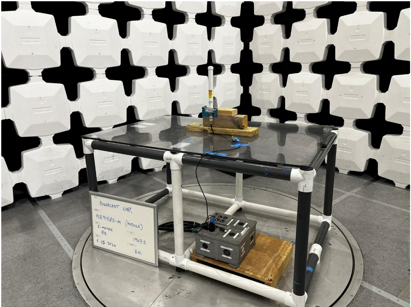
Antenna #3: PE510M1013, Radiated Emissions, 30MHz to 1GHz, View 3
