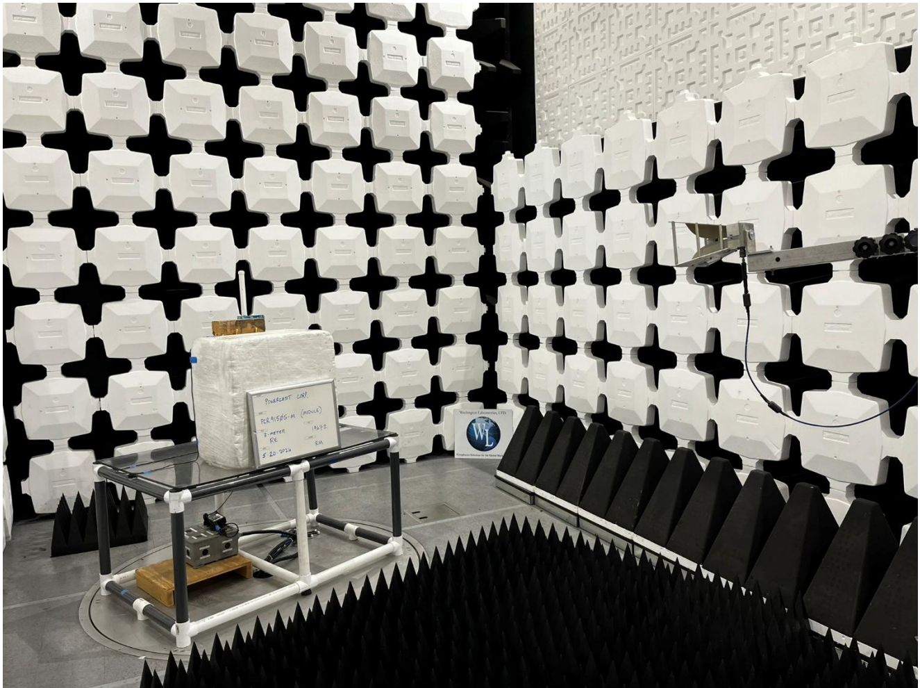
Antenna #3: PE510M1013, Radiated Emissions, 1GHz to 9.3GHz, View 1
