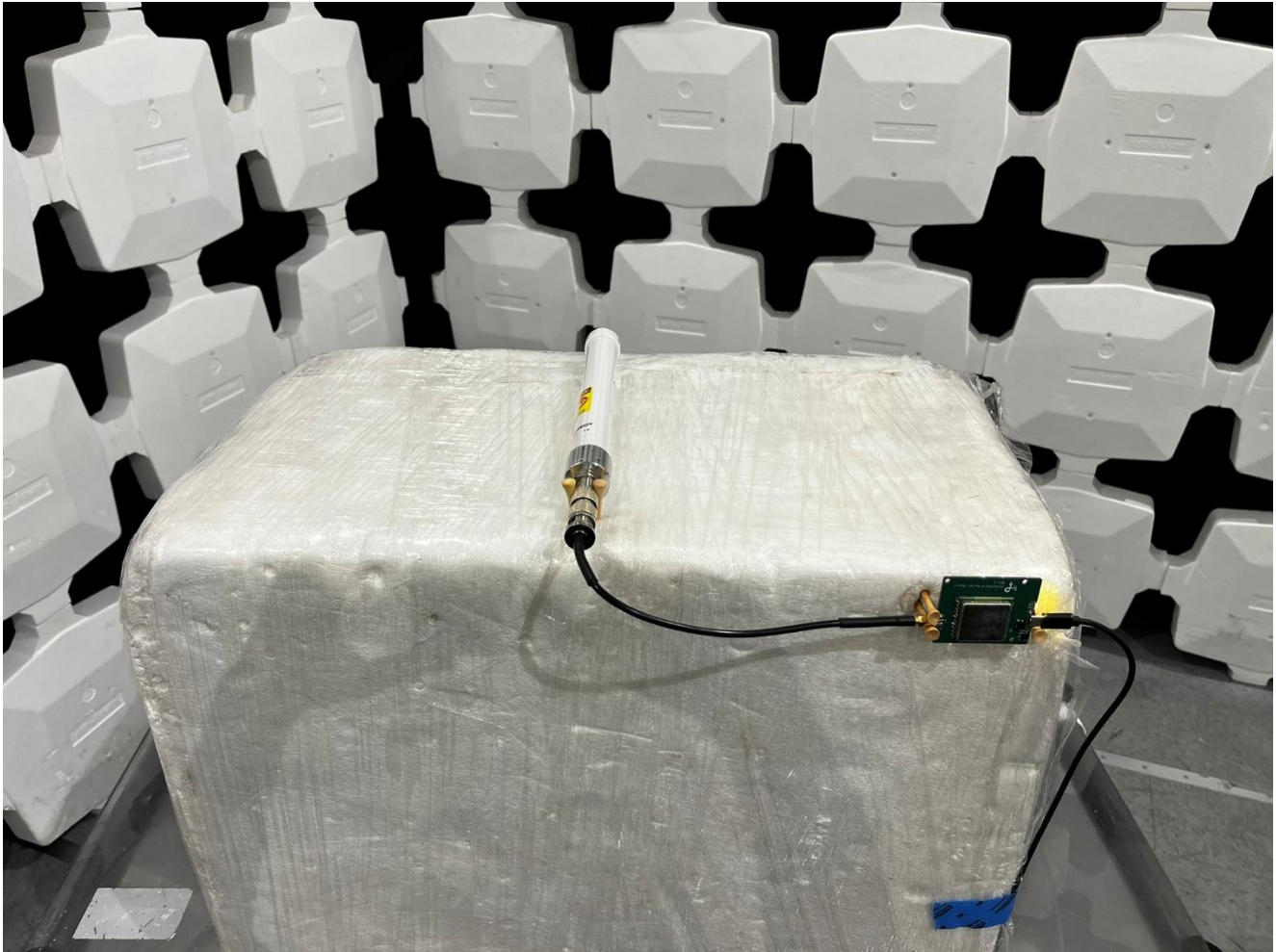
Antenna #3: PE510M1013, Radiated Emissions, 1GHz to 9.3GHz, View 4
