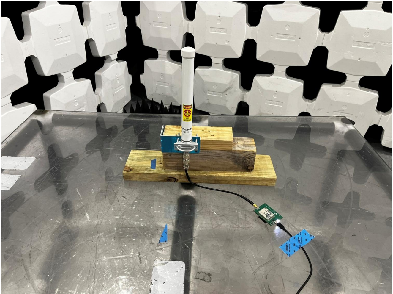
Antenna #3: PE510M1013, Radiated Emissions, 30MHz to 1GHz, View 4
