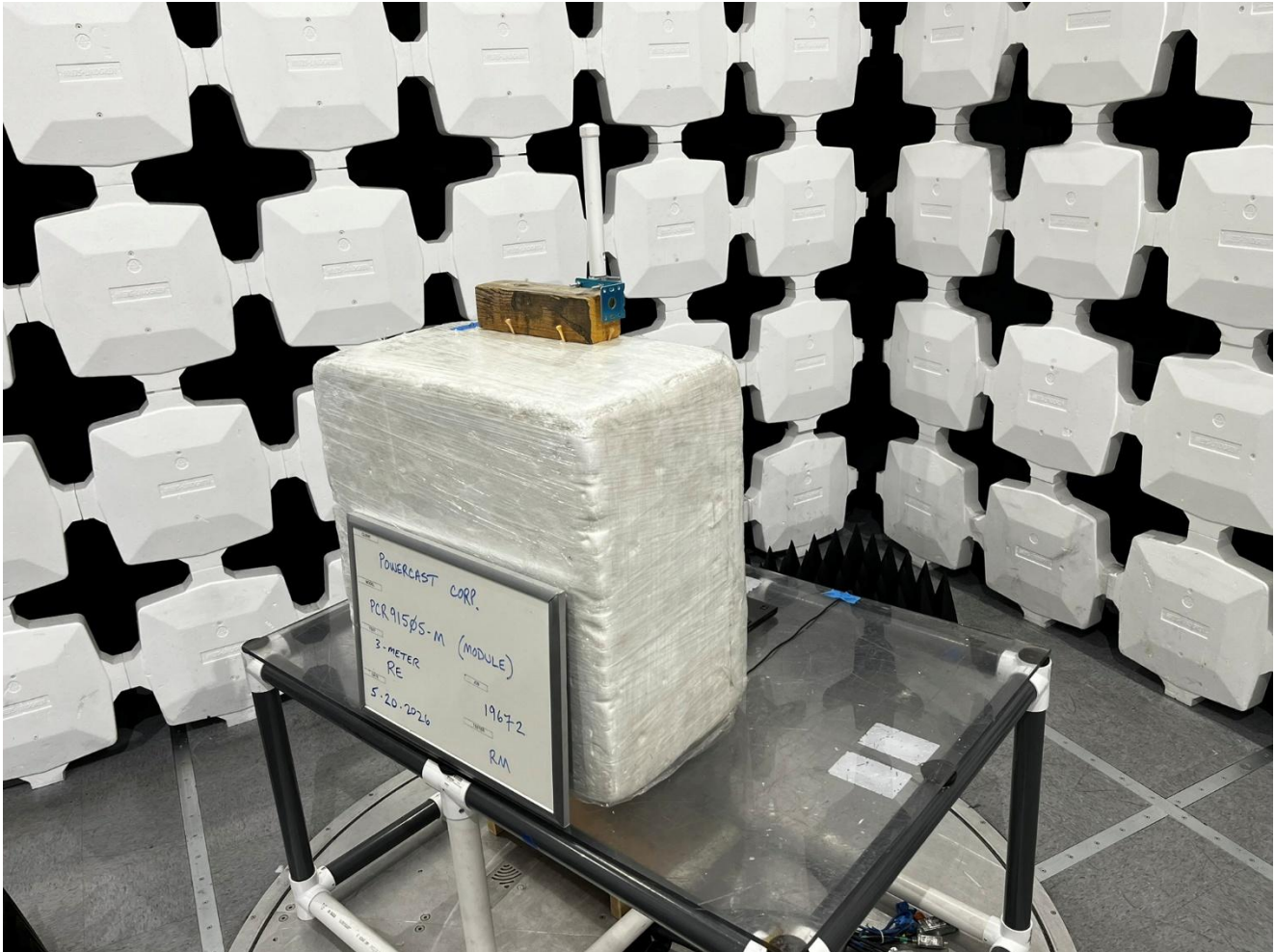
Antenna #3: PE510M1013, Radiated Emissions, 1GHz to 9.3GHz, View 2
