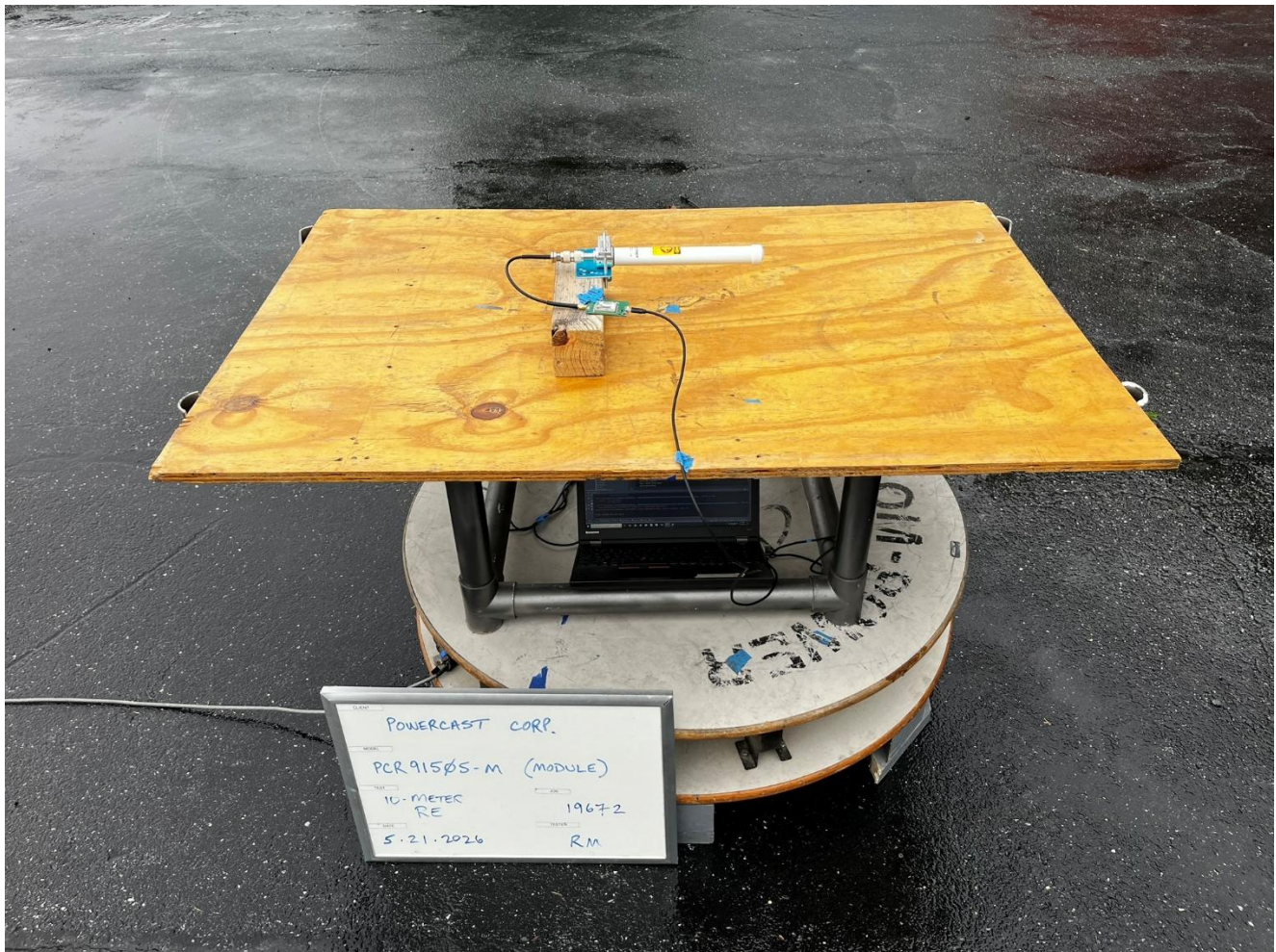
Antenna #3: PE510M1013, Radiated Emissions, 9kHz to 30MHz, View 3
