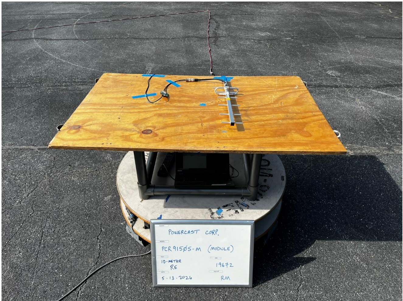
Antenna #4: PE51YA1009, Radiated Emissions, 9kHz to 30MHz, View 3
