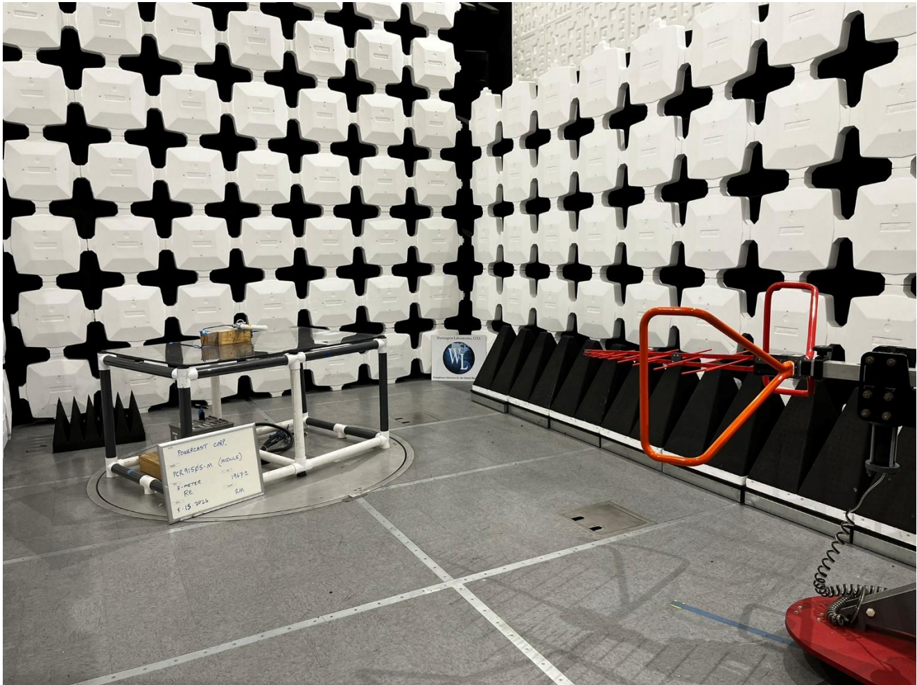
Antenna #3: PE510M1013, Radiated Emissions, 30MHz to 1GHz, View 1
