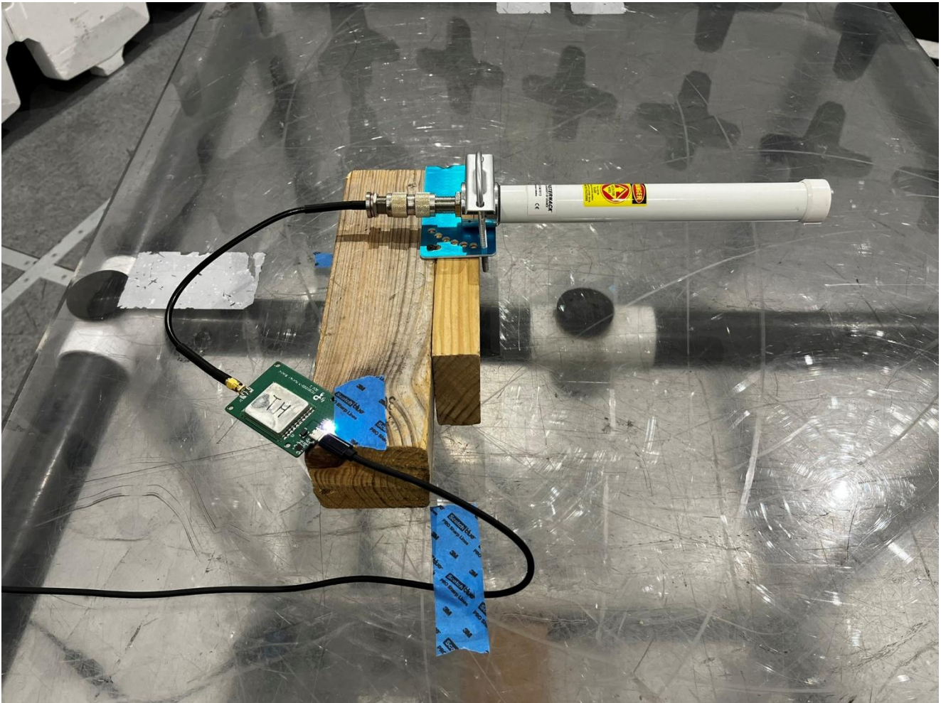
Antenna #3: PE510M1013, Radiated Emissions, 30MHz to 1GHz, View 2
