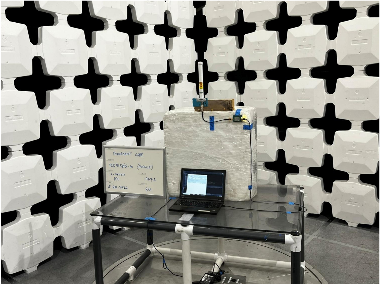
Antenna #3: PE510M1013, Radiated Emissions, 1GHz to 9.3GHz, View 3
