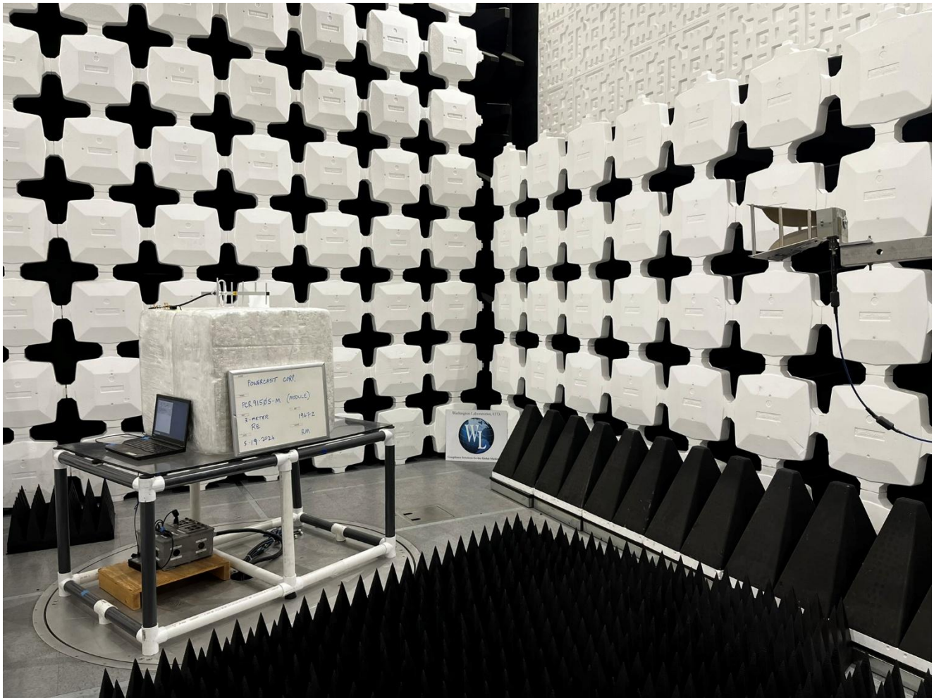
Antenna #4: PE51YA1009, Radiated Emissions, 1GHz to 9.3GHz, View 1
