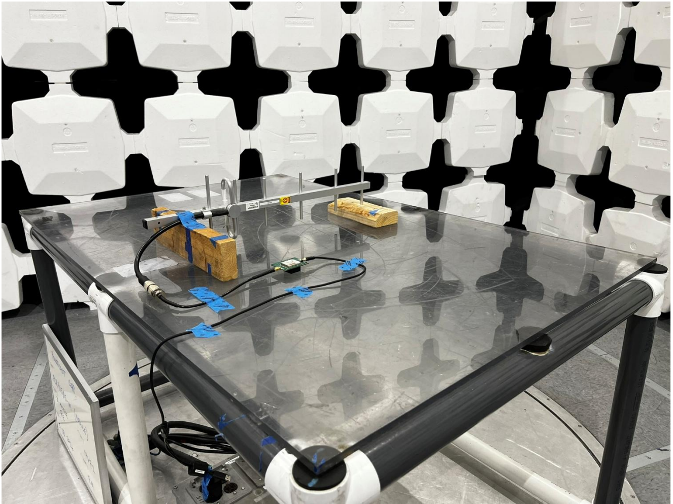
Antenna #4: PE51YA1009, Radiated Emissions, 30MHz to 1GHz, View 2
