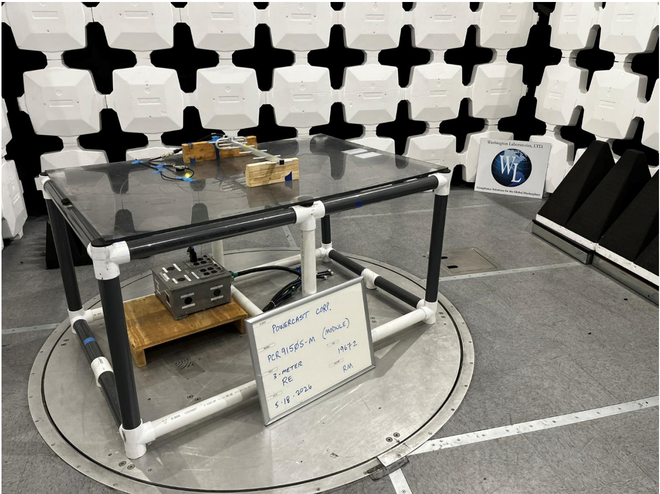
Antenna #4: PE51YA1009, Radiated Emissions, 30MHz to 1GHz, View 3
