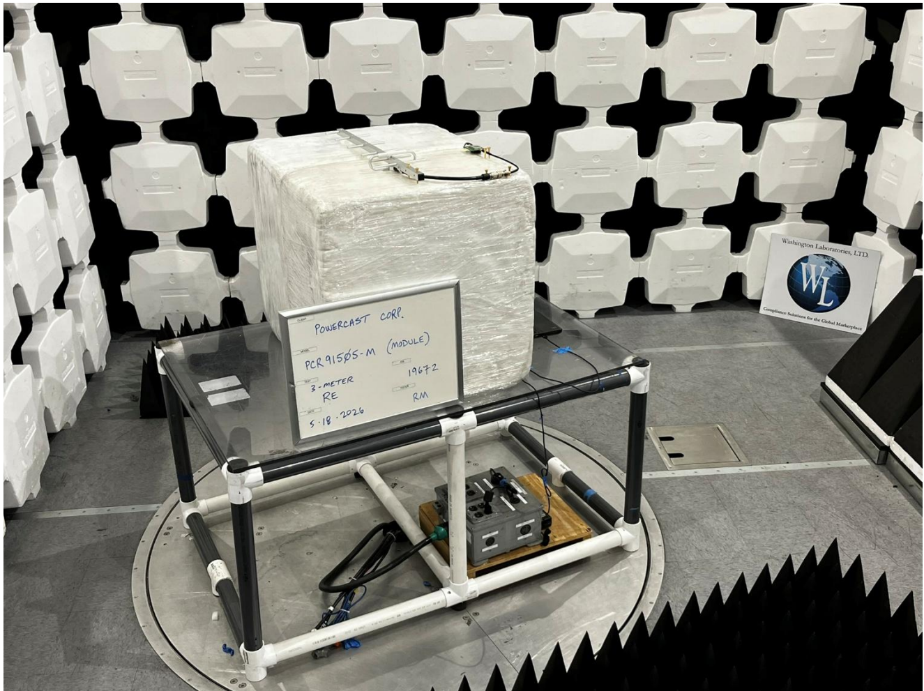
Antenna #4: PE51YA1009, Radiated Emissions, 1GHz to 9.3GHz, View 3
