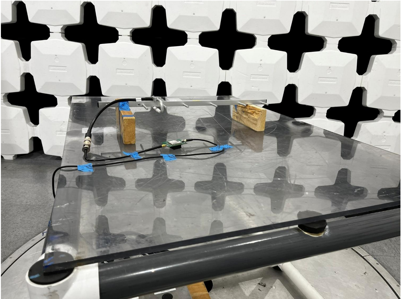
Antenna #4: PE51YA1009, Radiated Emissions, 30MHz to 1GHz, View 4
