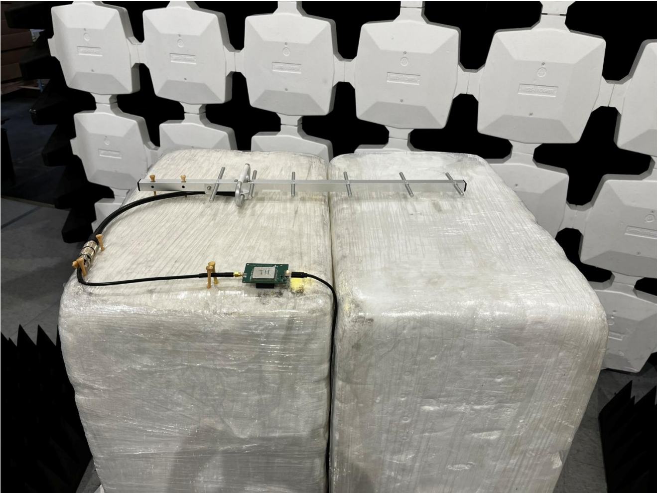
Antenna #4: PE51YA1009, Radiated Emissions, 1GHz to 9.3GHz, View 4
