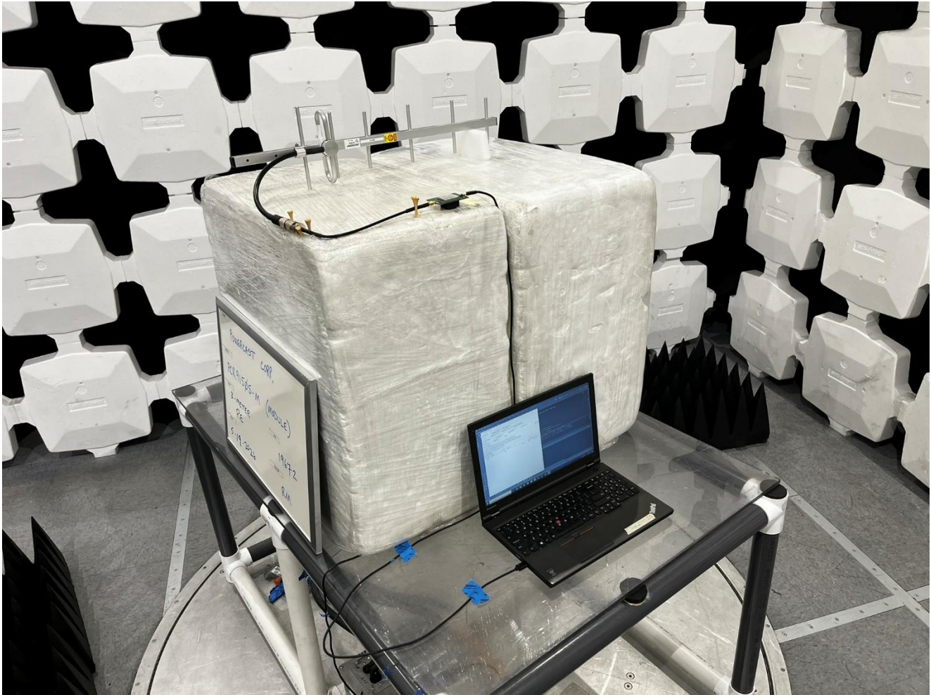
Antenna #4: PE51YA1009, Radiated Emissions, 1GHz to 9.3GHz, View 2
