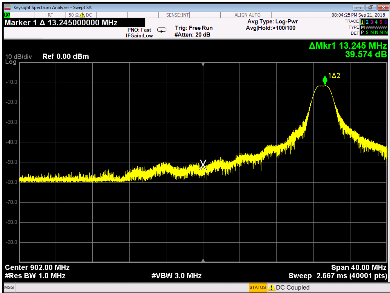
Mid Data Rate Lower Band Edge
