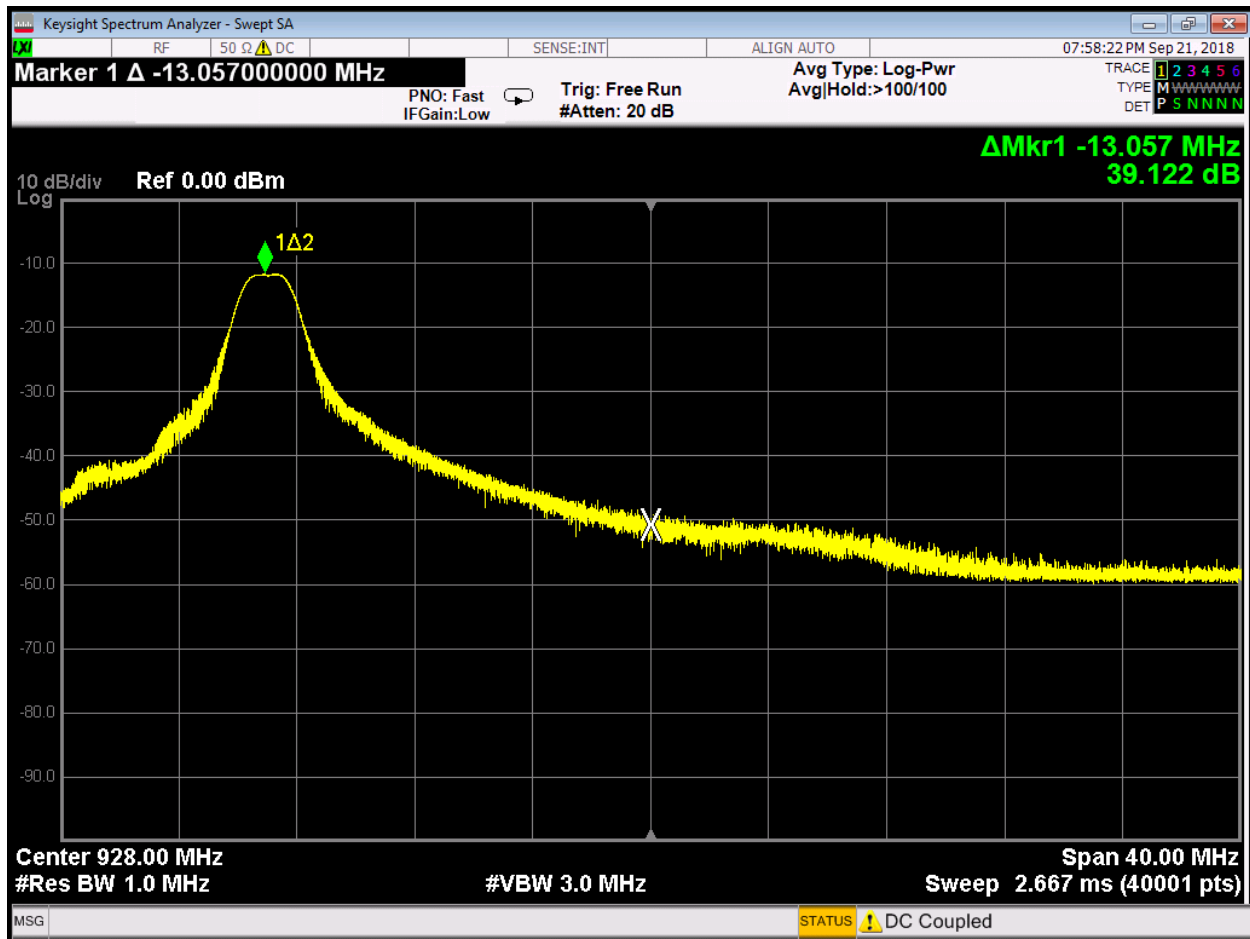
High Data Rate Upper Band Edge
