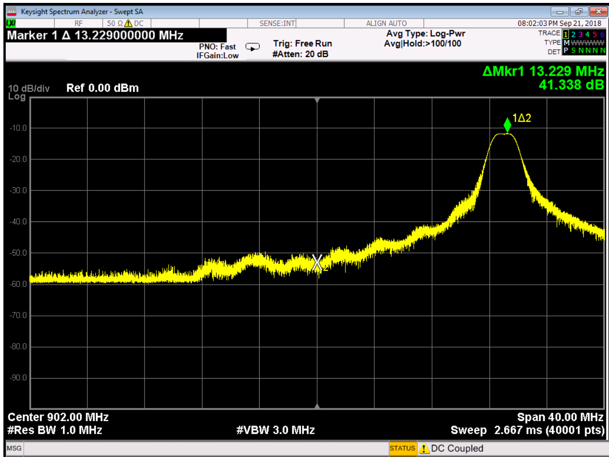
High Data Rate Lower Band Edge
