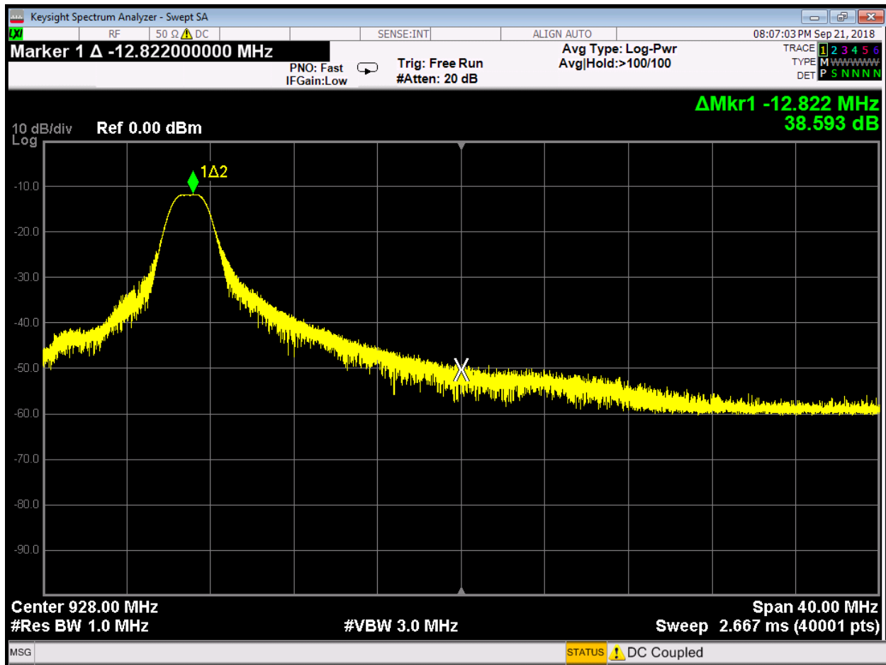
Mid Data Rate Upper Band Edge
