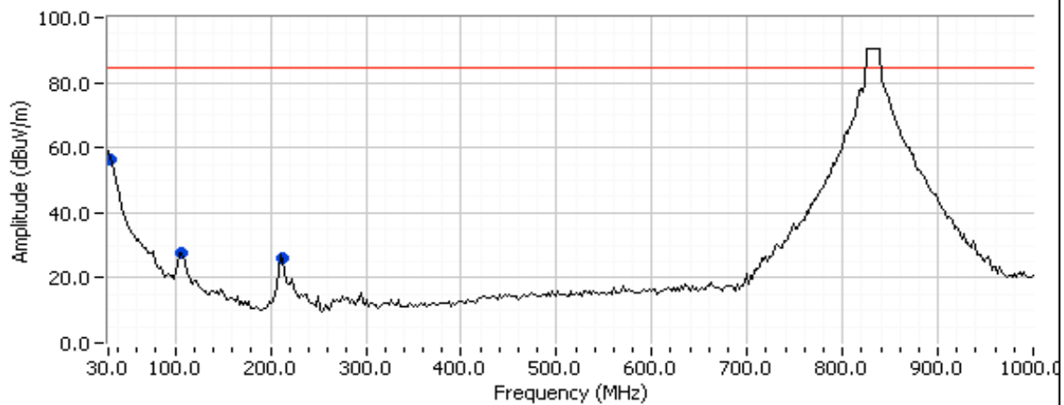
Band 5 3 channels RF low
