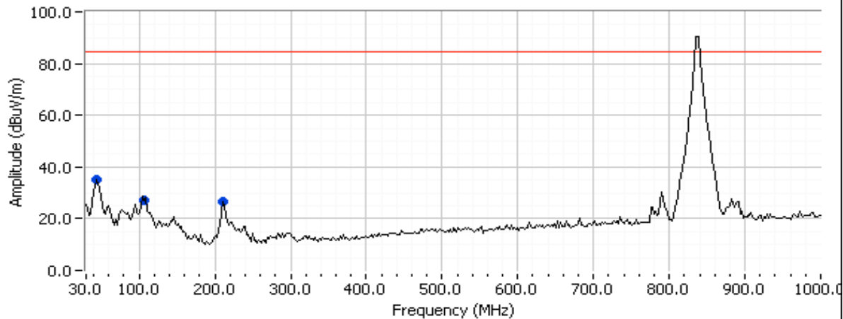
Band 5 Single MID channel
