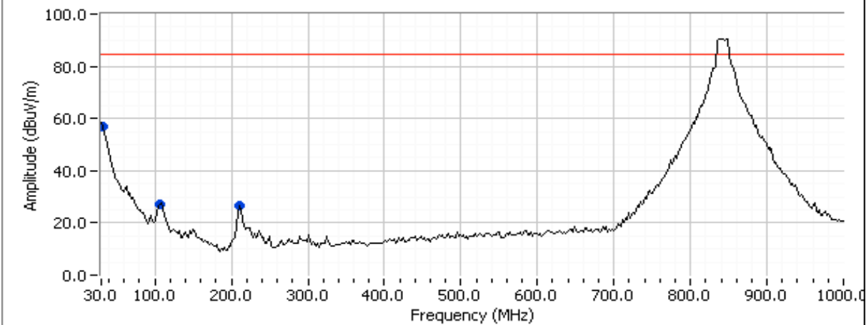
Band 5 Three RF chain high
