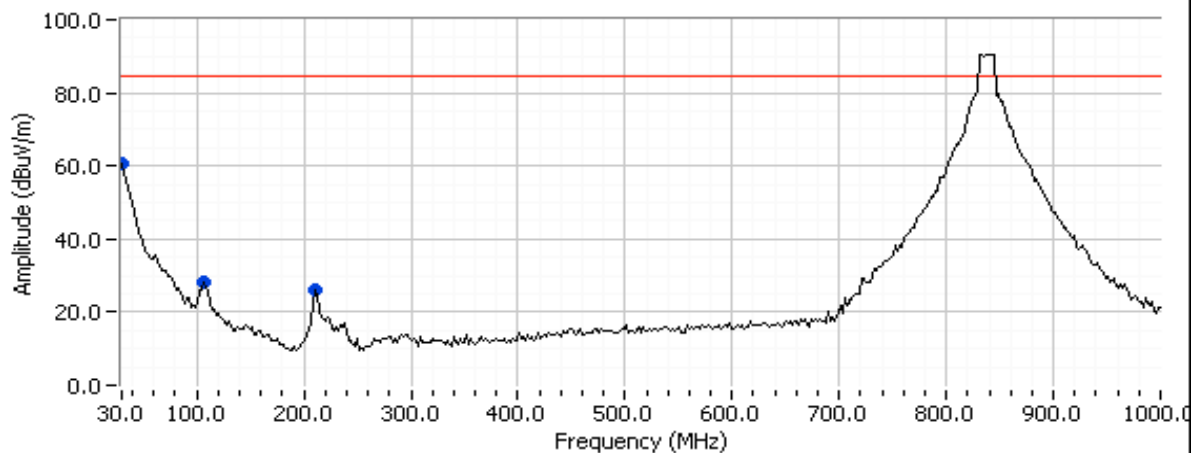
Band 5 Three RF chain MID
