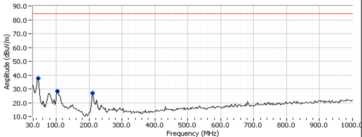
Band 2 Three RF Chain MID
