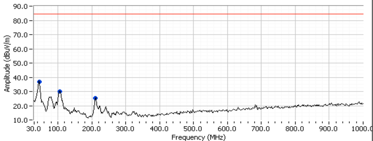
Band 2 Single highest channel
