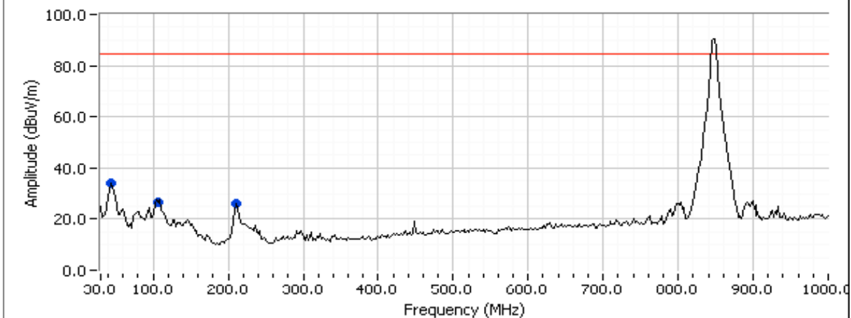
Band 5 single highest chain
