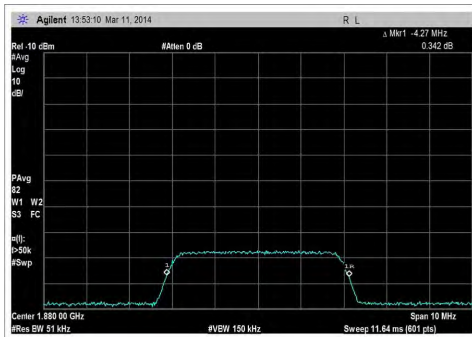
UL_1850-1915MHz_41AWGN_input
