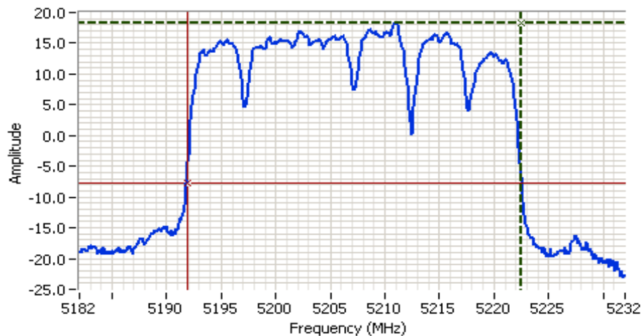
NU Ch Freq 5207 MHz @ 30 MHz Bandwidth
