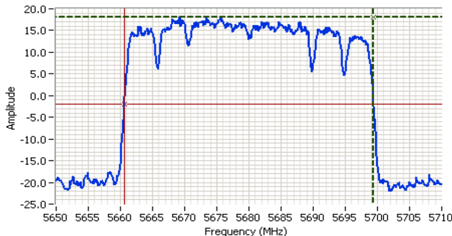
Channel Frequency 5680 MHz with 40 MHz Bandwidth
