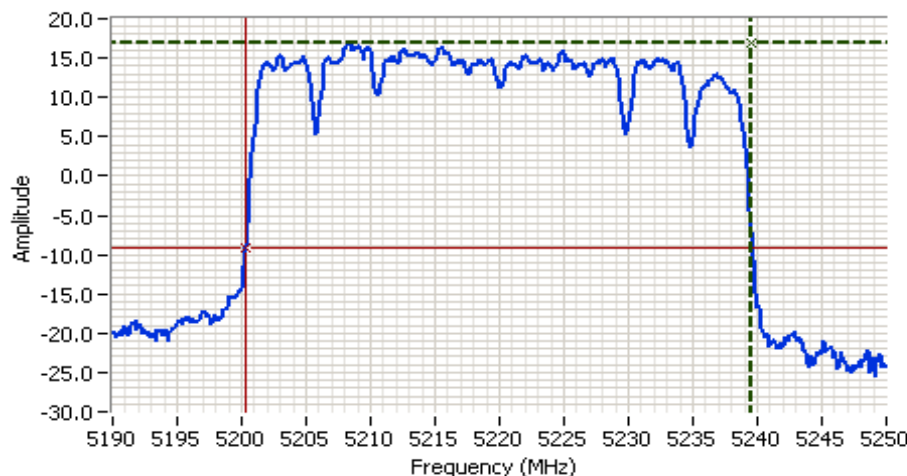
NU Ch Freq 5220 MHz @ 40 MHz Bandwidth
