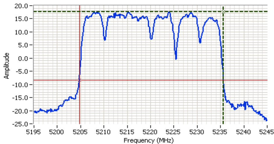
NU Ch Freq 5220 MHz @ 30 MHz Bandwidth
