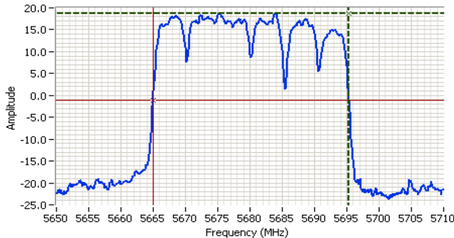
Channel Frequency 5680 MHz with 30 MHz Bandwidth
