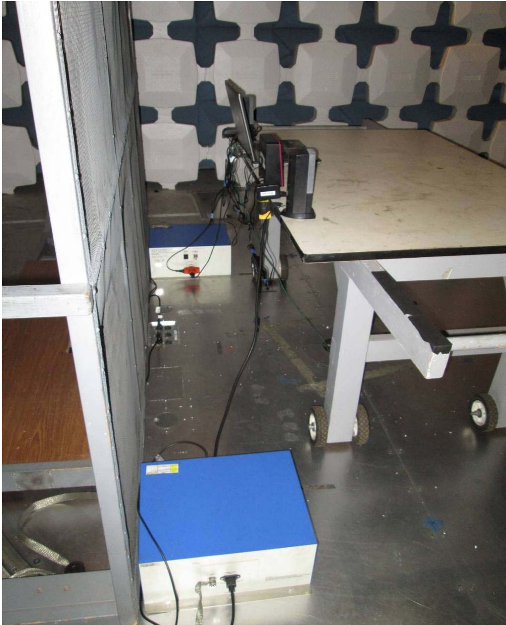
Test Configuration Photograph #2 (Conducted Emissions - Power Port)
