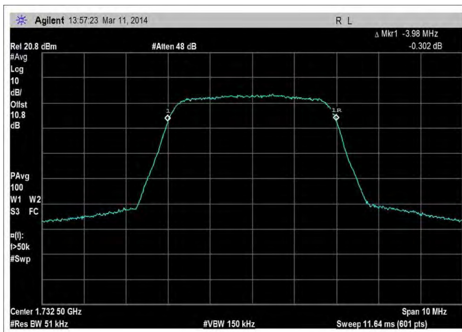
UL_1710-1755MHz_41AWGN_output
