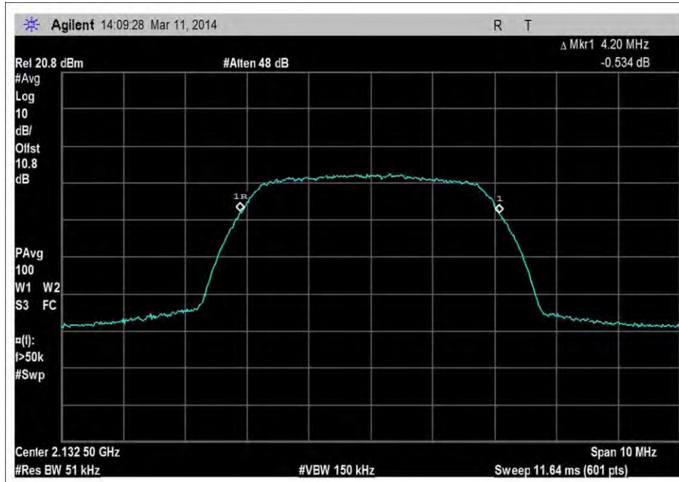
DL_2110-2155MHz_41AWGN_output
