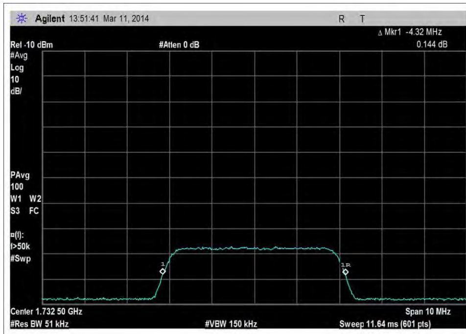
UL_1710-1755MHz_41AWGN_input
