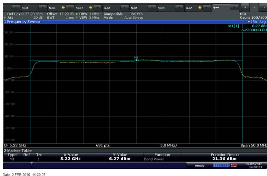
UNII 1 40MHz Bandwidth Mid Channel 5220 MHz
