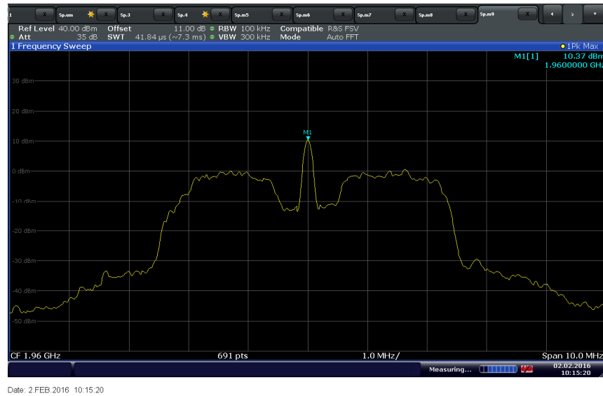
Downlink Mid Channel 120VAC @ 20°C
