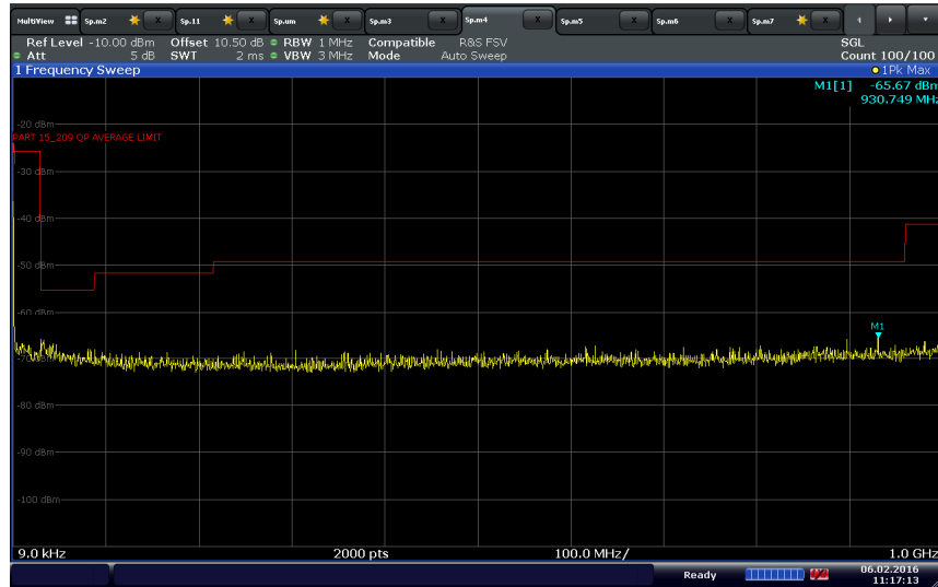
UNII 1 30MHz Bandwidth Middle Channel 5220 MHz Below 1GHz
