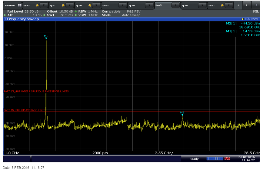
UNII 1 30MHz Bandwidth Middle Channel 5220 MHz Above 1GHz
