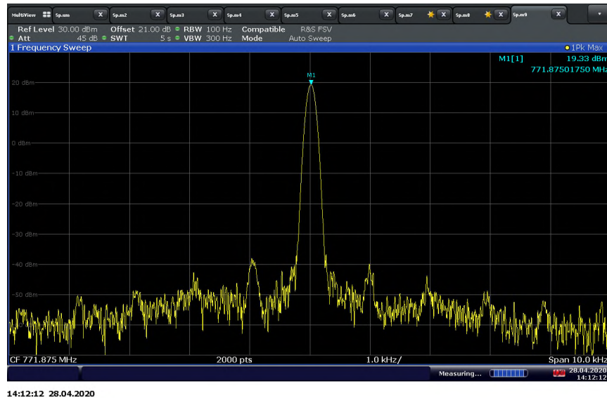
700MHz Narrowband Public Safety Downlink Middle Channel @ 20°C Nominal Voltage (The same as the inject CW signal)
