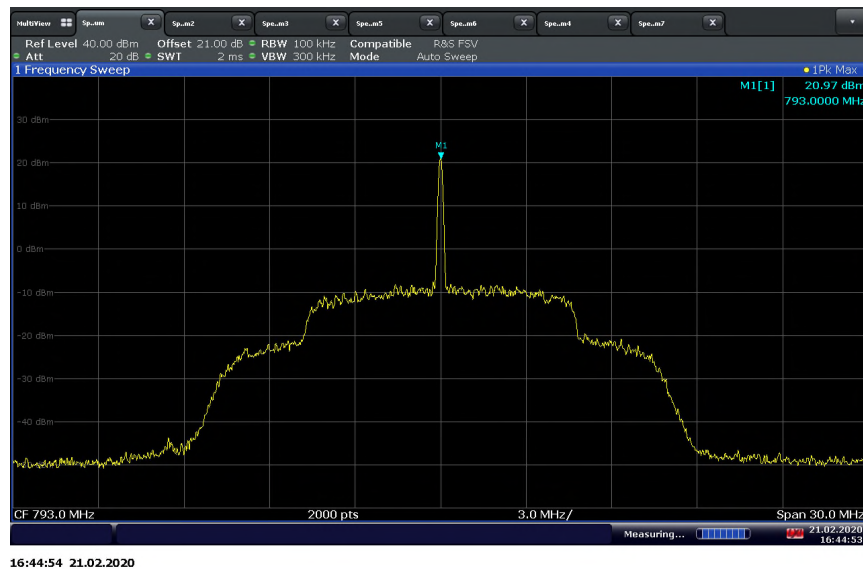
LTE Band 14 Uplink Middle Channel 120VAC @ 20°C
