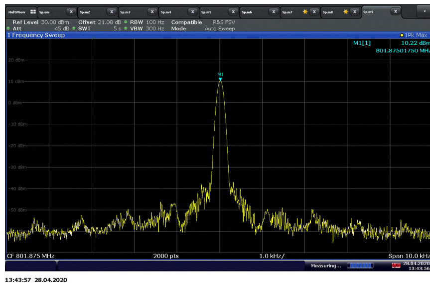
700MHz Narrowband Public Safety Uplink Middle Channel @ 20°C Nominal Voltage (The same as the inject CW signal)
