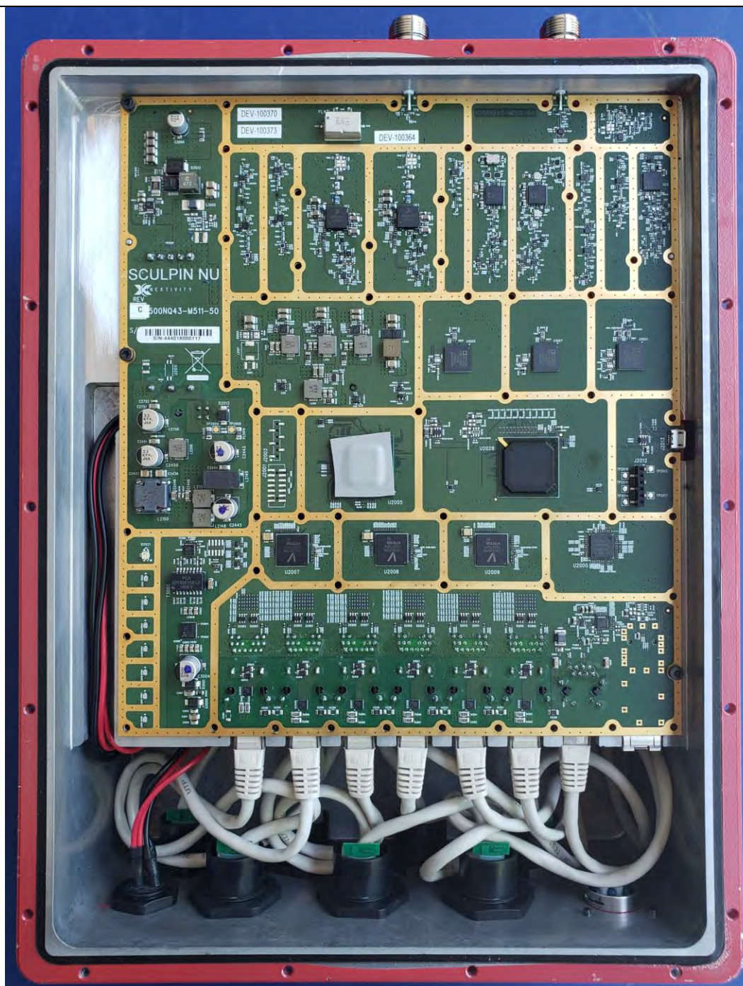
Cover off, PCB side 1
