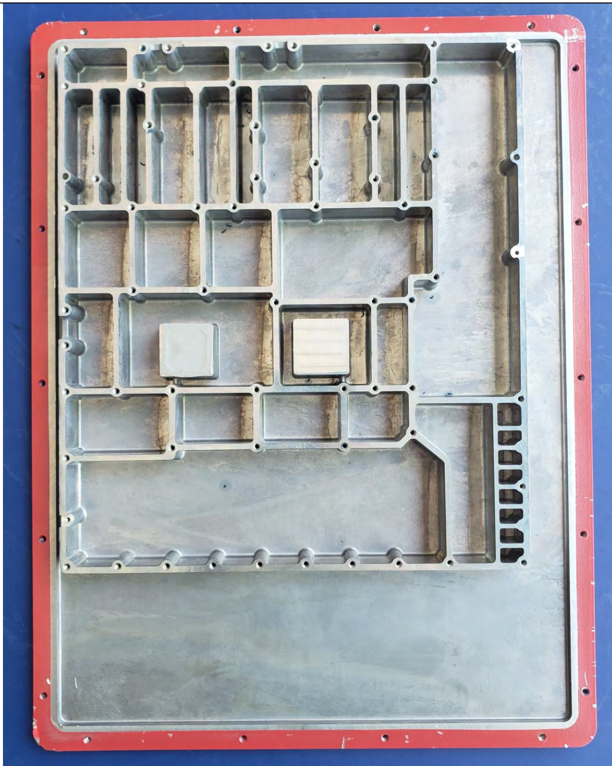
Housing_Top_Internal
