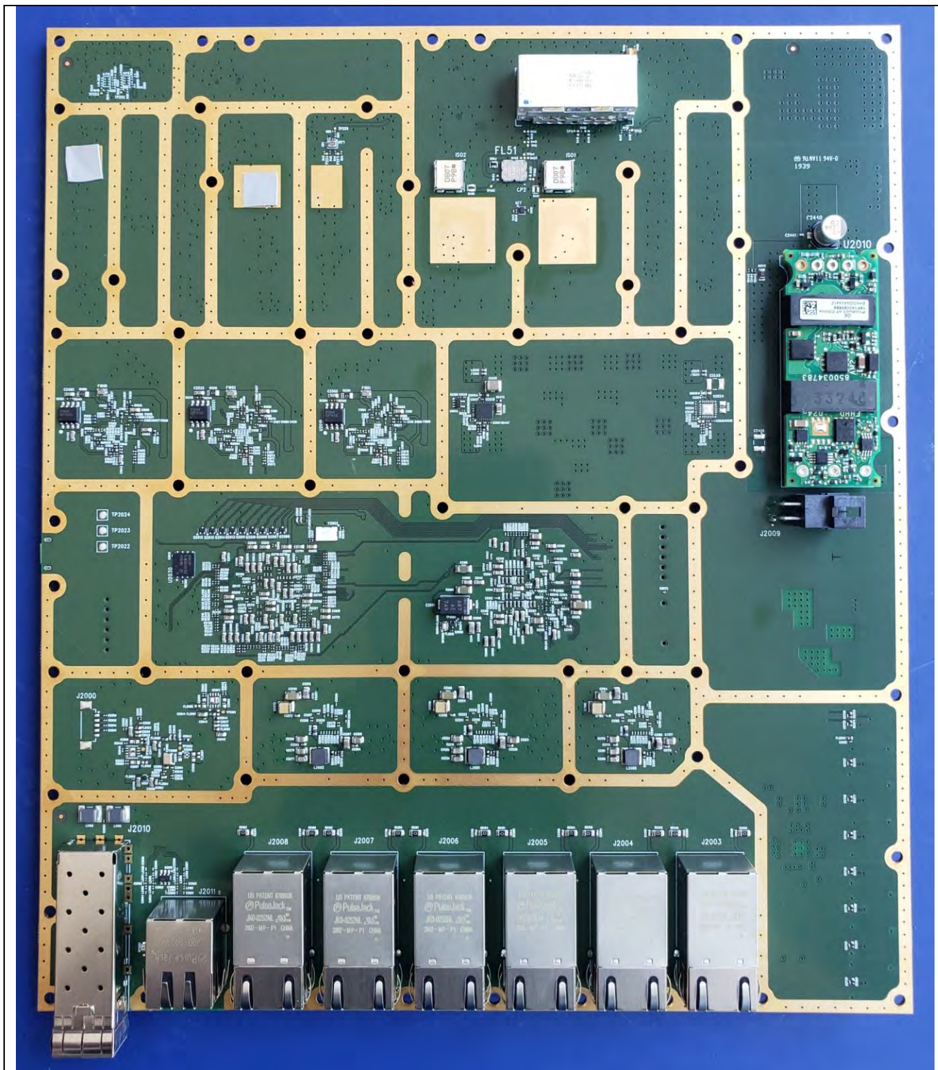
PCB side 2
