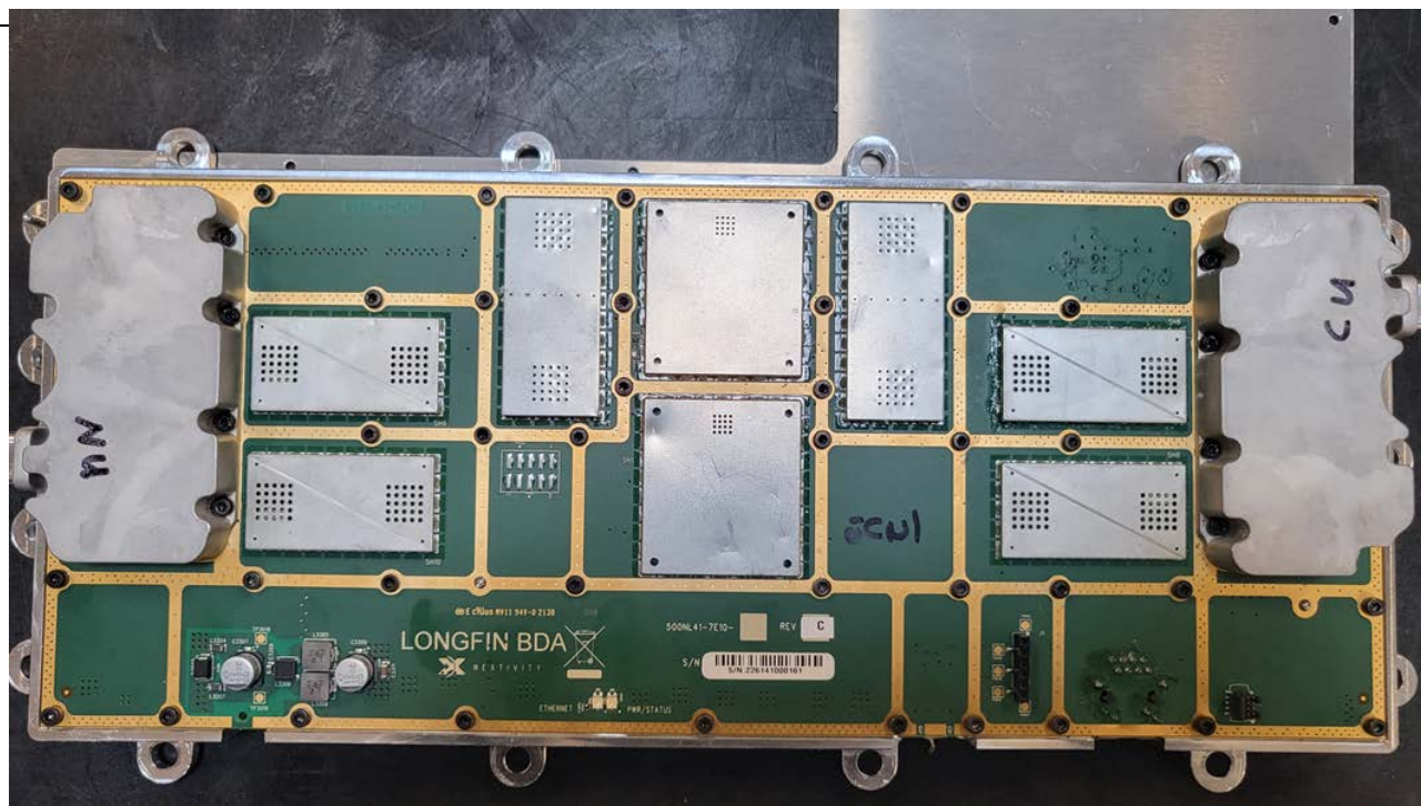
PCB_1 w/shields
