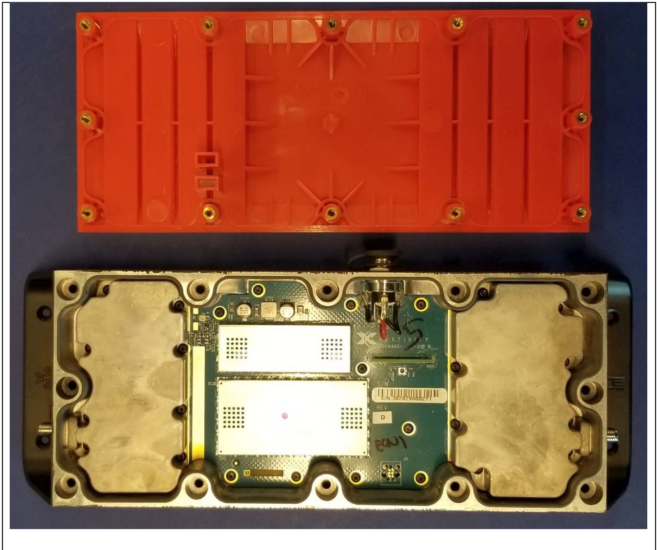
PCB side 1 / Top Cover
