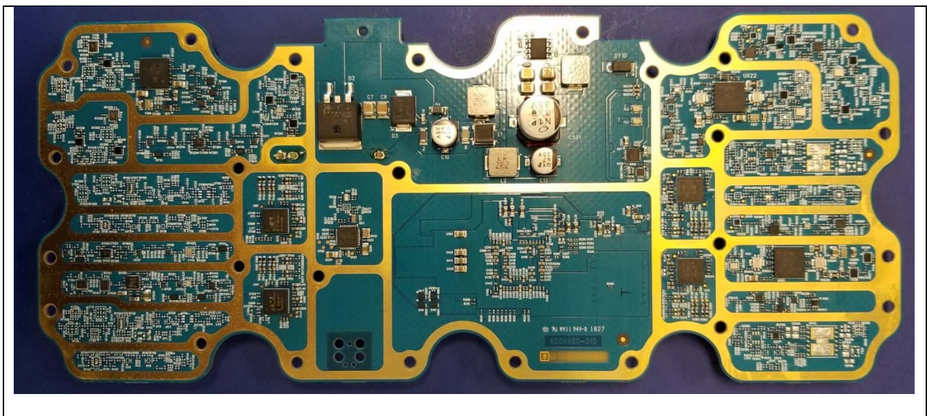
PCB side 2
