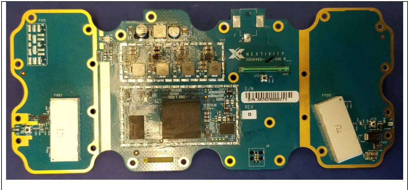
PCB side 1 (no shields)
