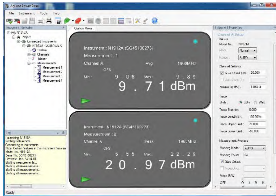
WCDMA Band 2_Downlink_5MHz Bandwidth_Mid Channel
