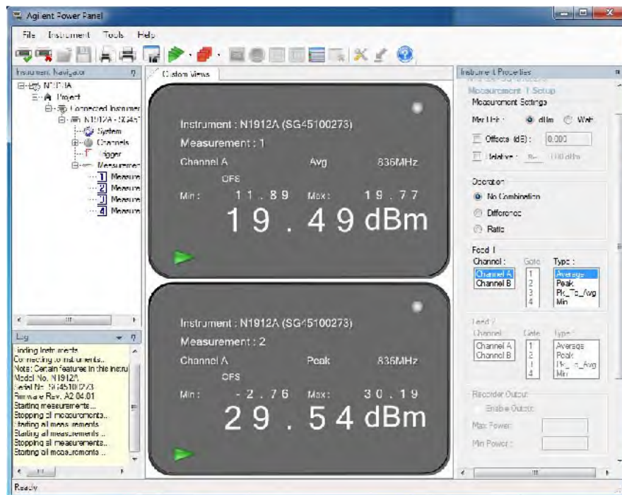
WCDMA Band 5_UpLink_5MHz Bandwidth_Mid Channel
