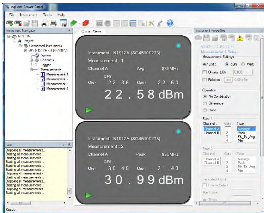
LTE Band 5_Uplink_5MHz Bandwidth_Mid Channel
