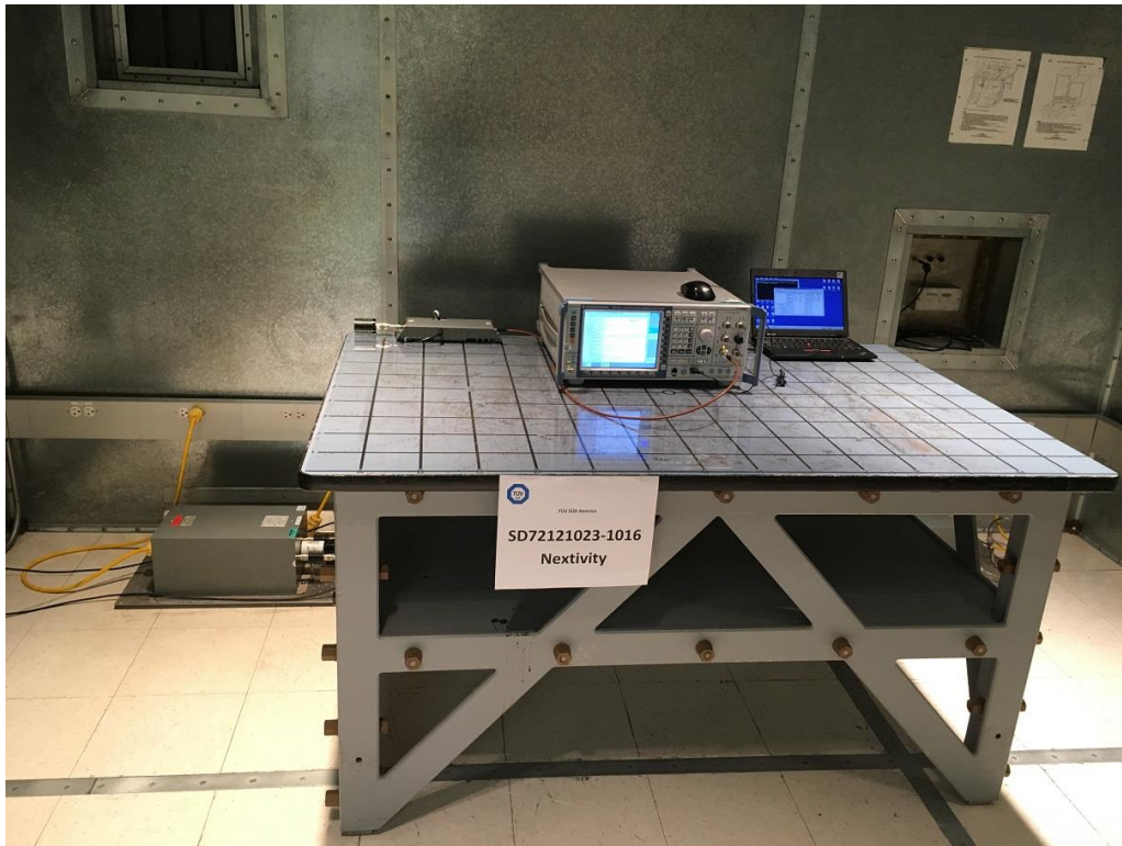
Conducted Testing
