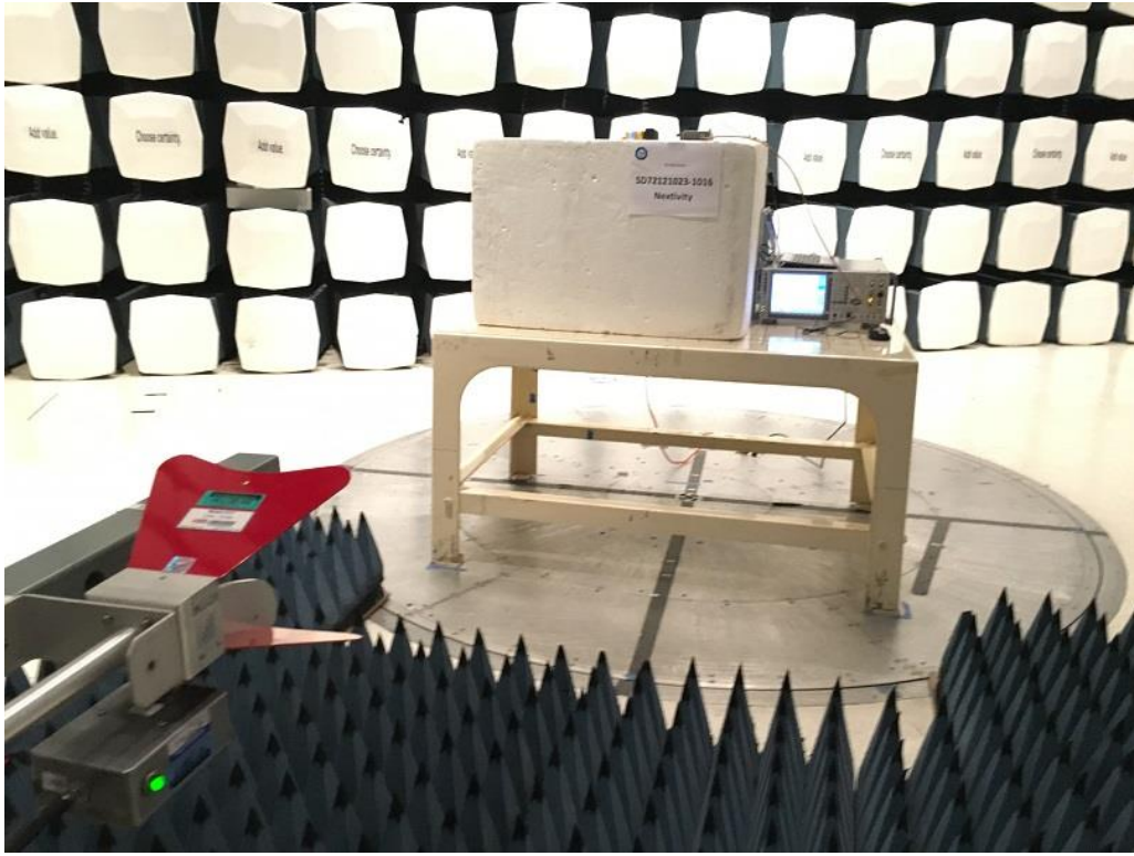
Radiated Emissions Above 1GHz Front
