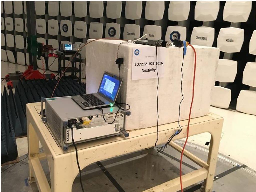
Radiated Emissionsv Above 1GHz Rear
