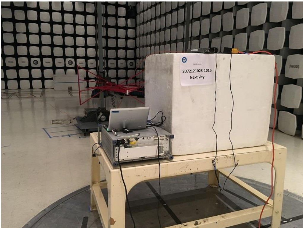
Radiated Emissions Below 1GHz Rear
