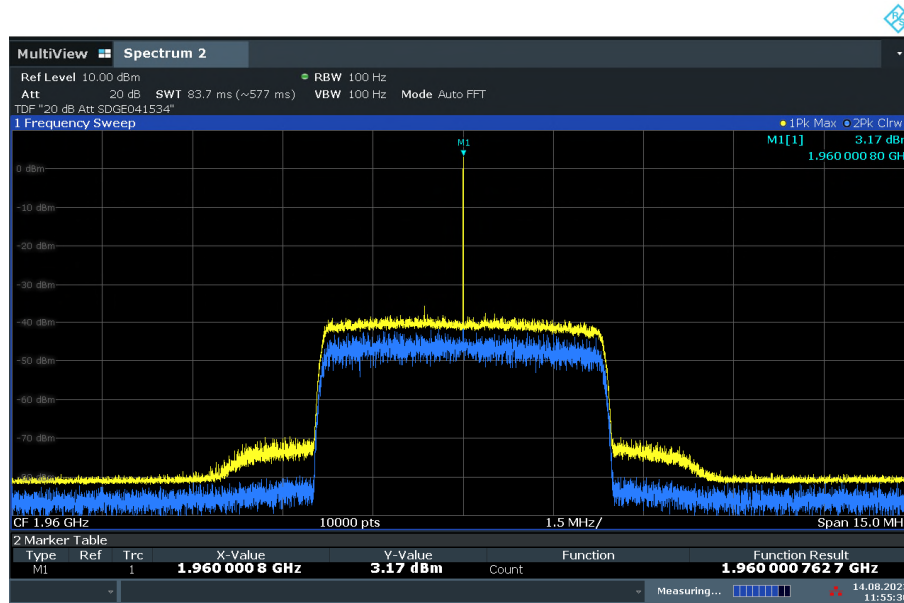
LTE B2 Downlink Middle Channel 120VAC @ 20°C
