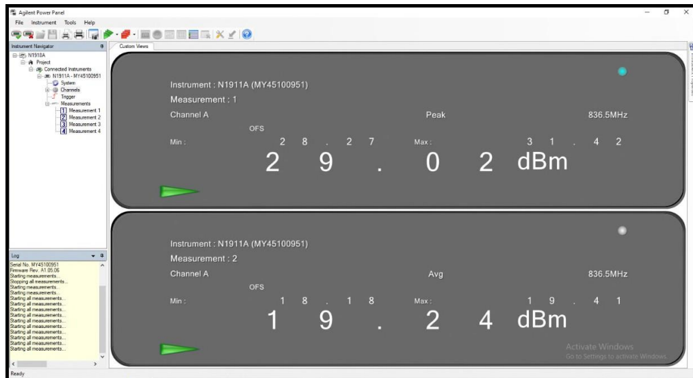
LTE Band 5 Uplink 5 MHz Bandwidth Middle Channel
