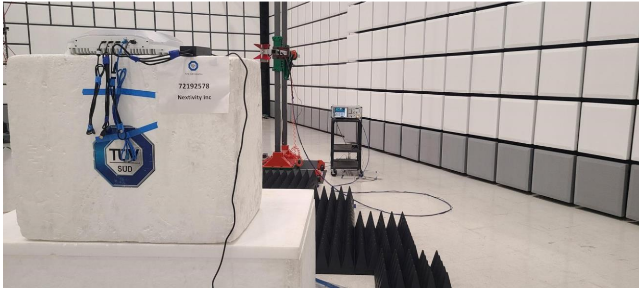
Radiated Spurious Emissions Test Setup 1GHz to 18GHz
