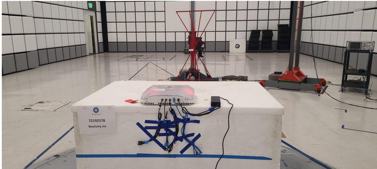
Radiated Spurious Emissions Test Setup 30MHz to 1GHz
