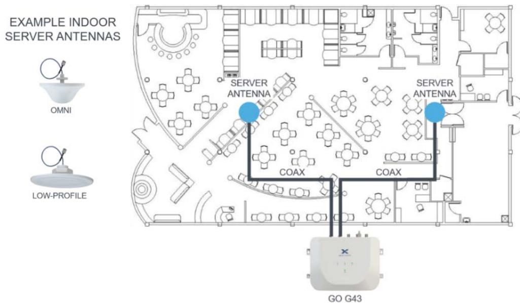
Two Server Antenna Ports, each feeding one antenna
