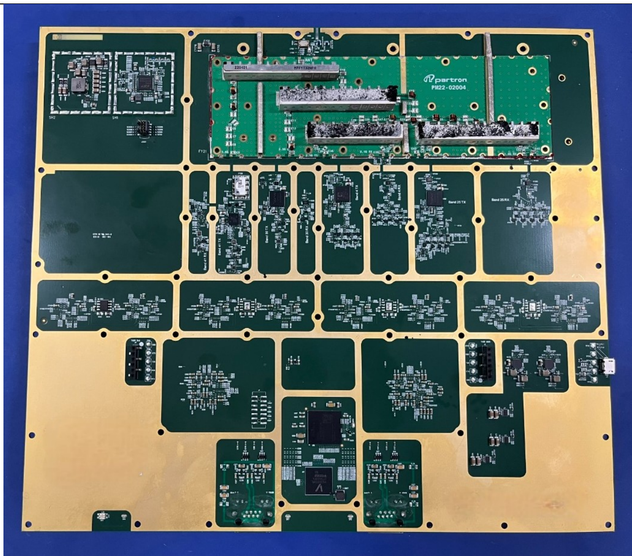
PCB Side 1_Radio
