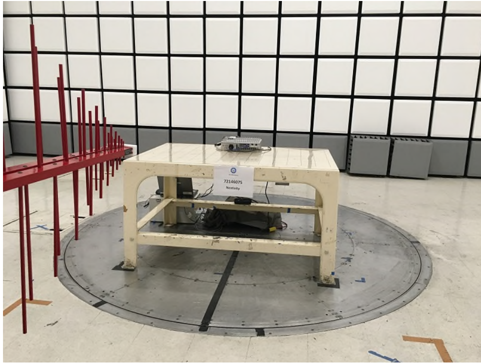
NU Intermodulation Radiated Emissions Below 1GHz Front
