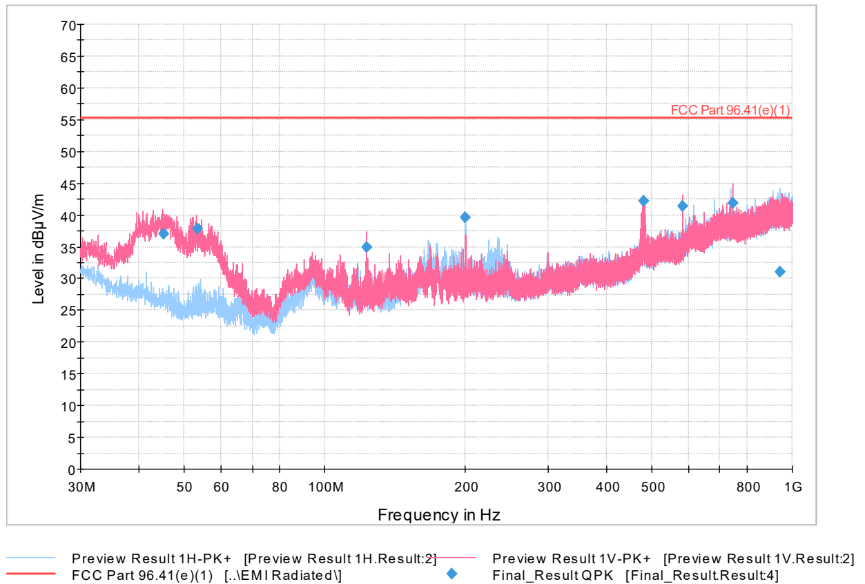
Full Spectrum
