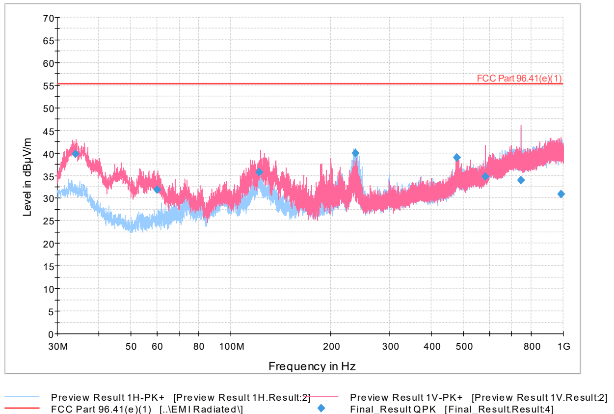
Full Spectrum
