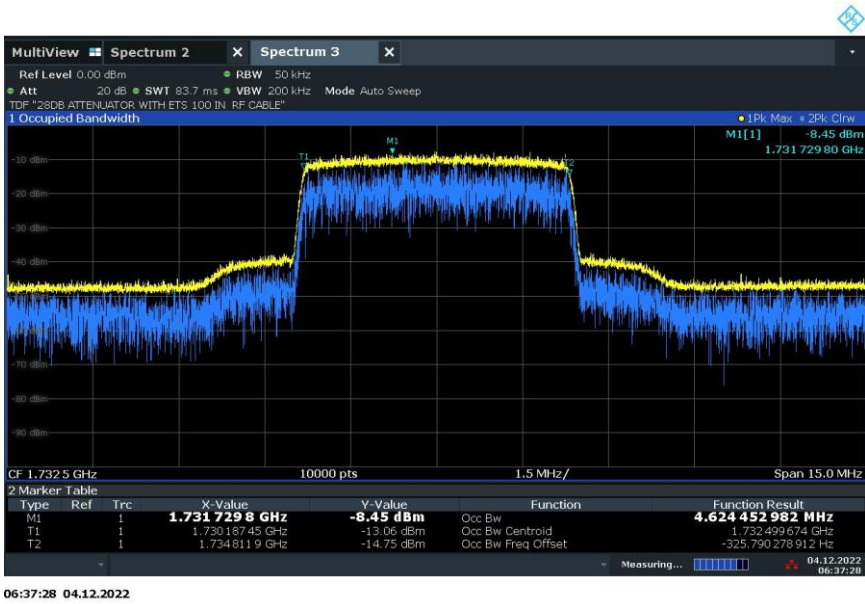
LTE Band 4 Uplink Middle Channel OBW 120VAC @ 20°C
