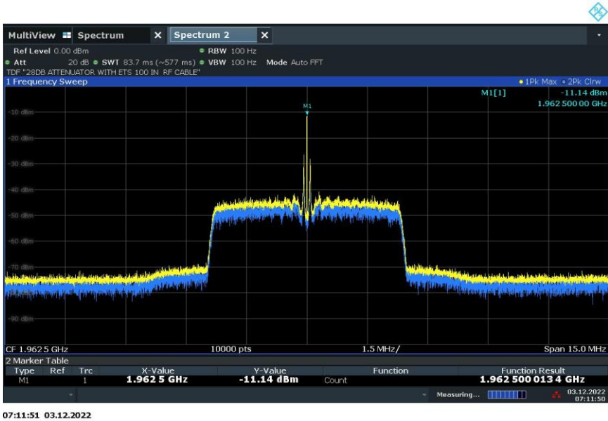
LTE B25 Downlink Middle Channel 120VAC @ 20°C
