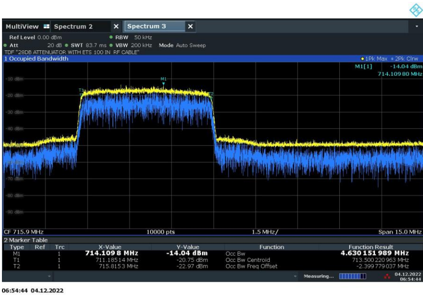
LTE B12 Uplink High Channel OBW @ 20°C Nominal Voltage
