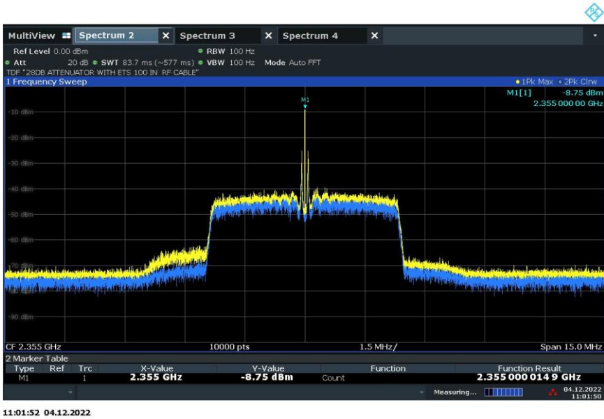
LTE B30 Downlink Middle Channel @ 40°C Nominal Voltage
