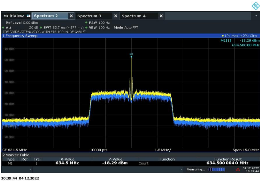
LTE B71 Downlink Middle Channel @ 40°C Nominal Voltage
