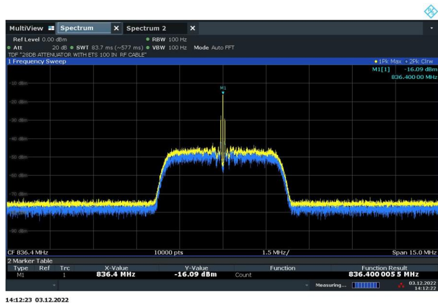
WCDMA B5 Uplink Middle Channel 120VAC @ -30°C
